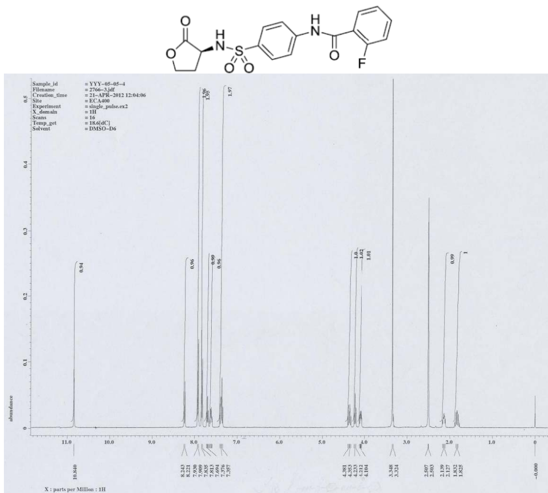
Figure S8. The ^1\text{H} -NMR spectrum of 5h .
