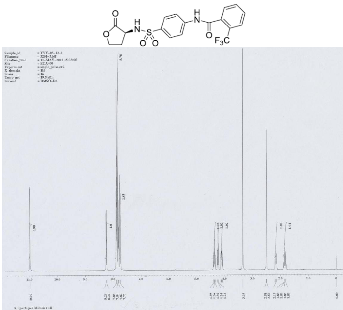
Figure S12. The ^1\text{H} -NMR spectrum of 5l .
