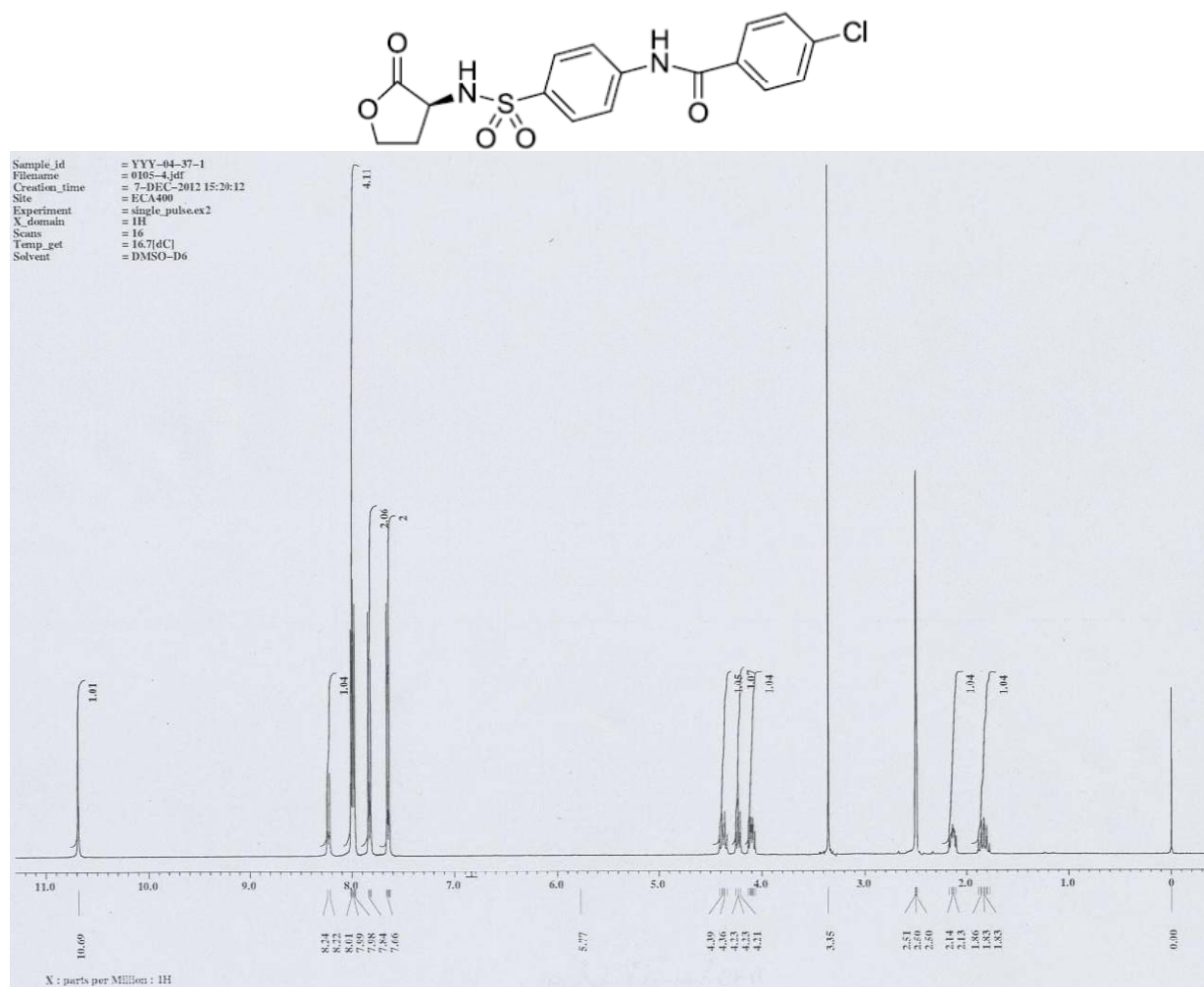
Figure S9. The ^1\text{H} -NMR spectrum of 5i .
