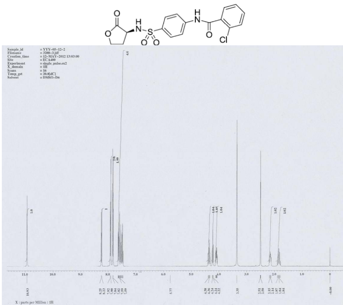
Figure S11. The ^1\text{H} -NMR spectrum of 5k .
