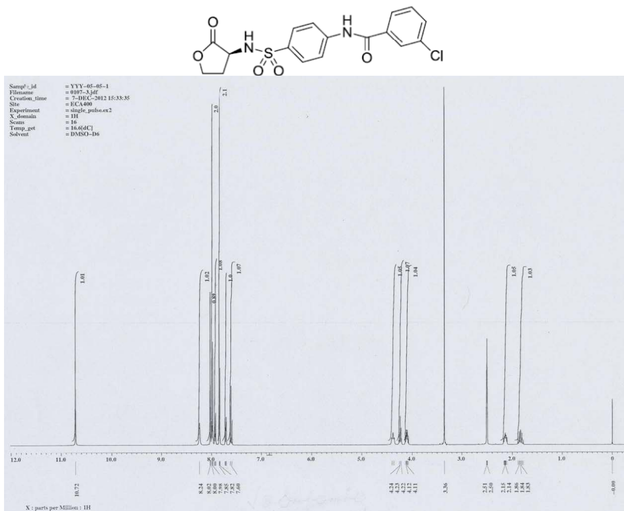
Figure S10. The ^1\text{H} -NMR spectrum of 5j .
