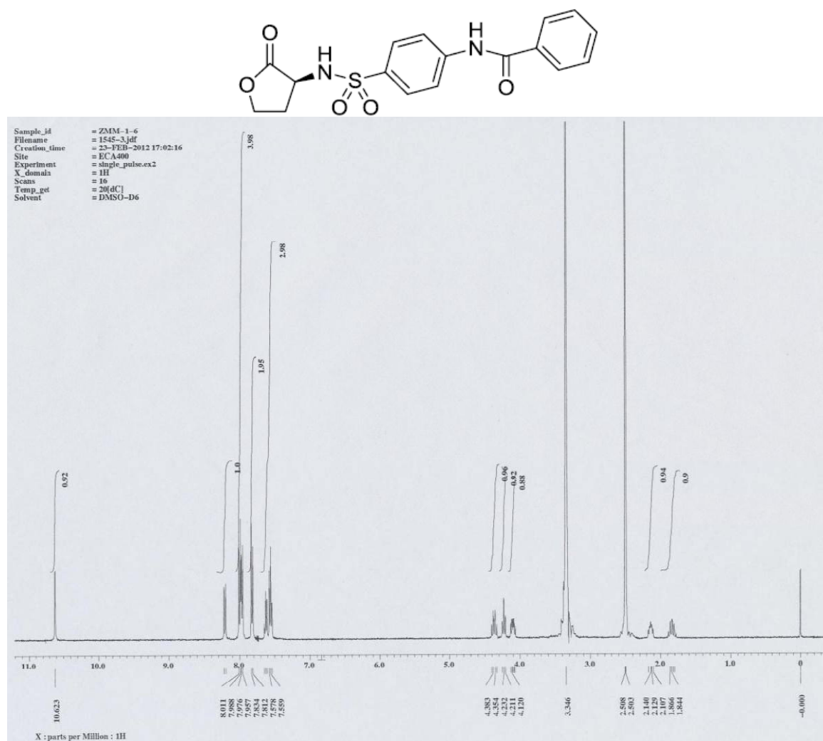
Figure S5. The ^1\text{H} -NMR spectrum of 5e .
