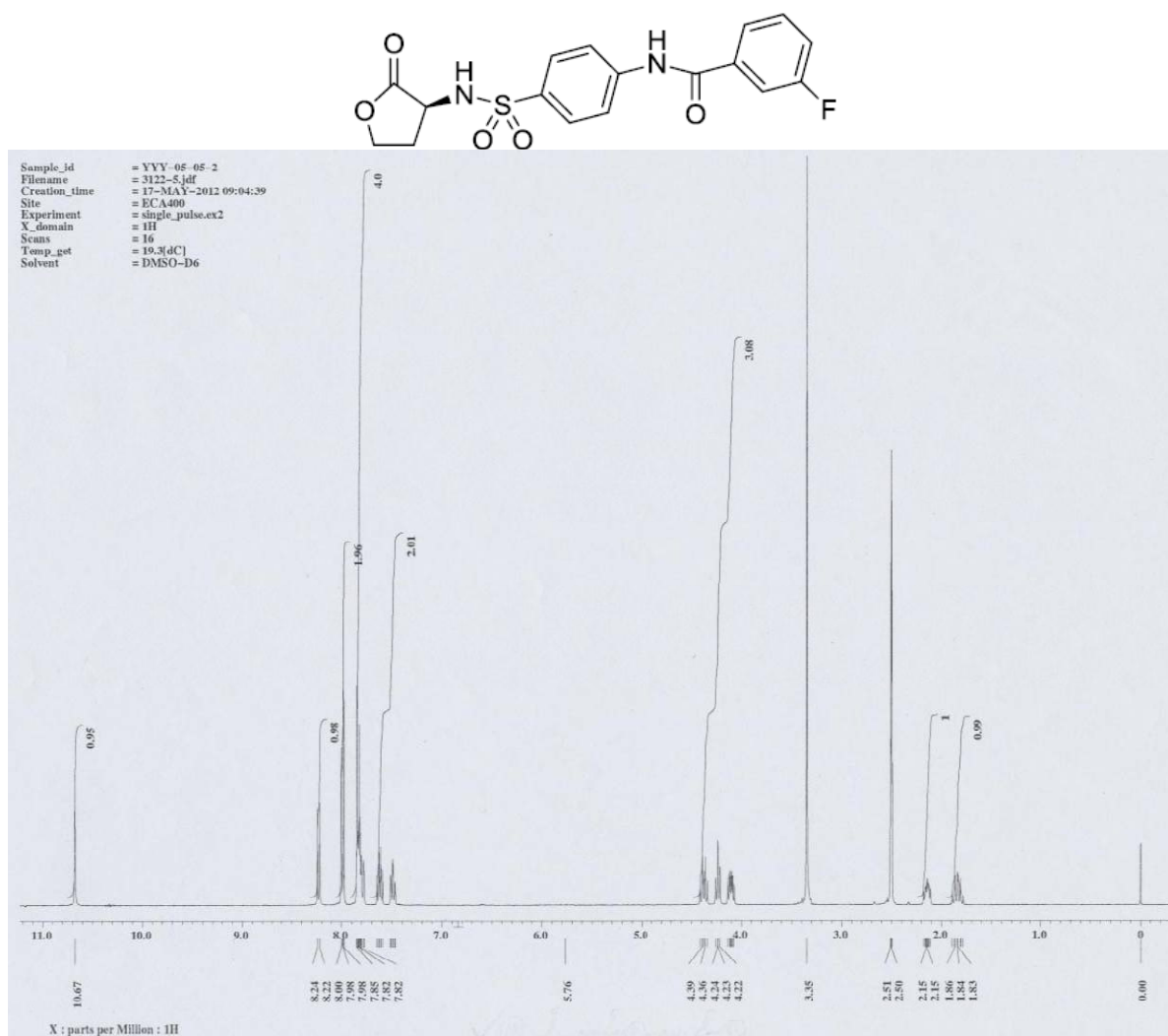
Figure S7. The ^1\text{H-NMR} spectrum of 5g .
