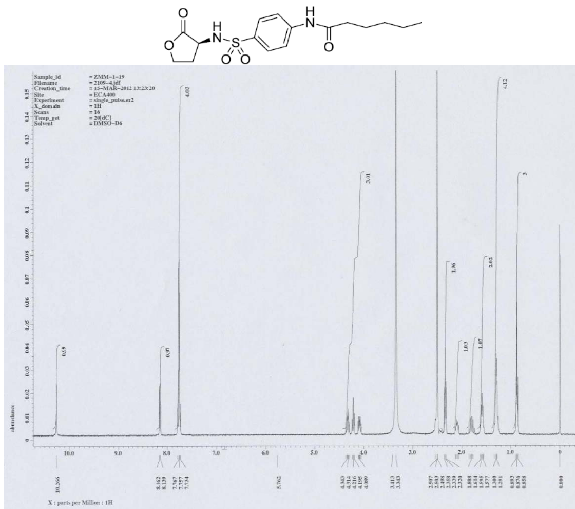
Figure S3. The ^1\text{H} -NMR spectrum of 5c .
