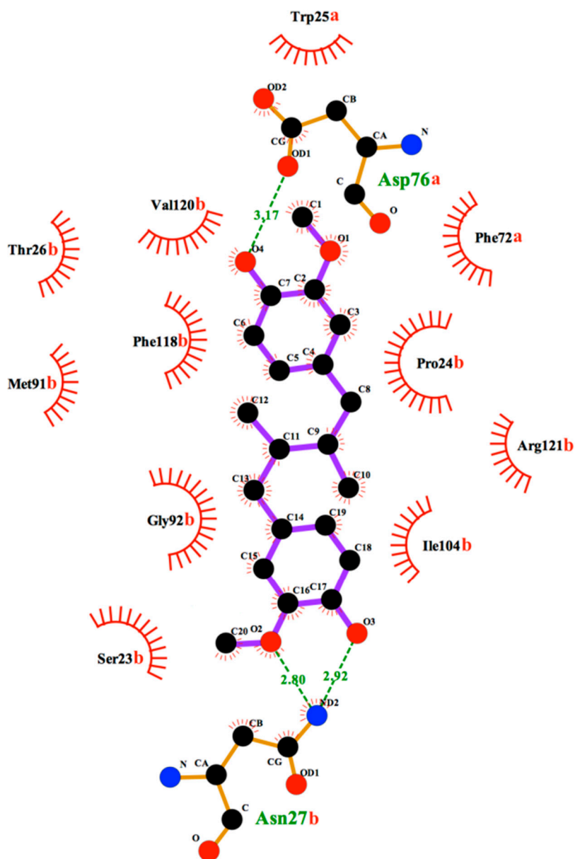
Figure S2. Predicted interactions of the MDGA molecule on the CoAt-Mt binding site by docking studies. The segmented lines represent hydrogen bond and its distance and the residues with red lines means interactions by Van der Waals contacts.
