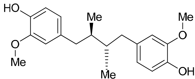
Figure S1. Lignan meso -dihydroguaiaretic acid with antimycobacterial activity.
