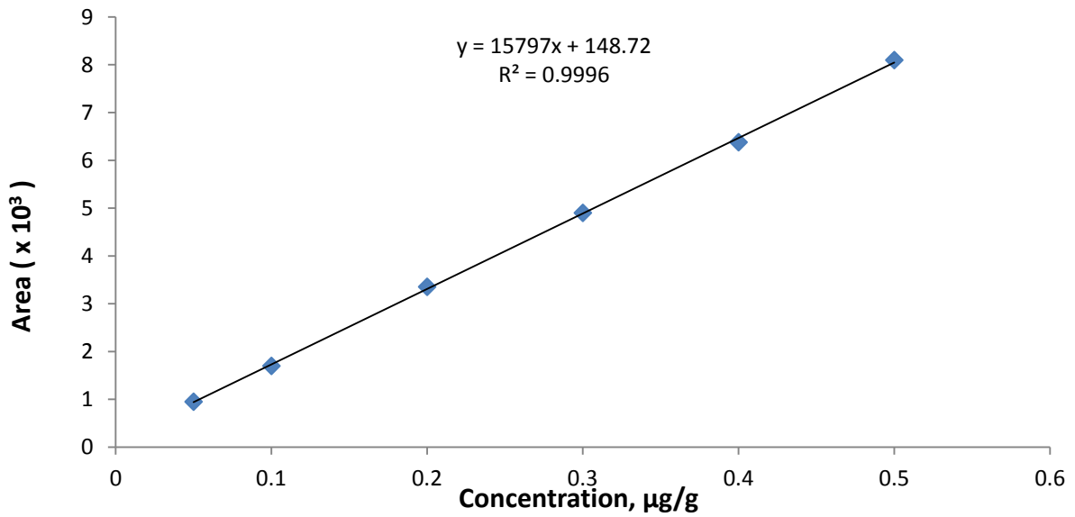
Figure S2. Calibration curve for Dihydrocapsaicin.
