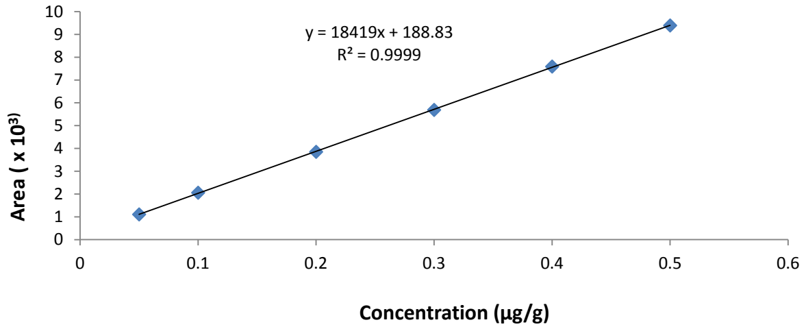
Figure S2. Calibration curve for Dihydrocapsaicin.
