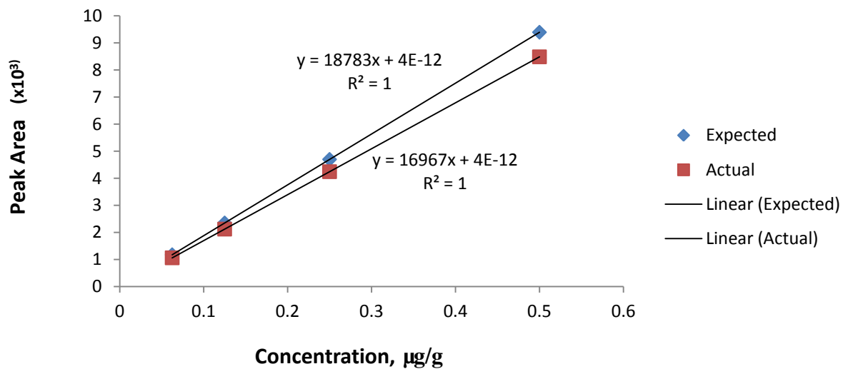
Figure S3. Expected and actual response plotted against expected concentrations for capsaicin.
