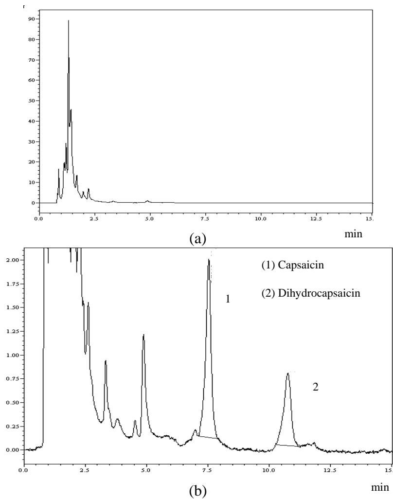
Figure S5. The chromatogram of an extracted solution of some genotypes. (a) Blank Sample (AVPP0803) – Non pungent; (b) AVPP0514 (Highly Pungent); and (c) C05573 (Very Highly Pungent).
