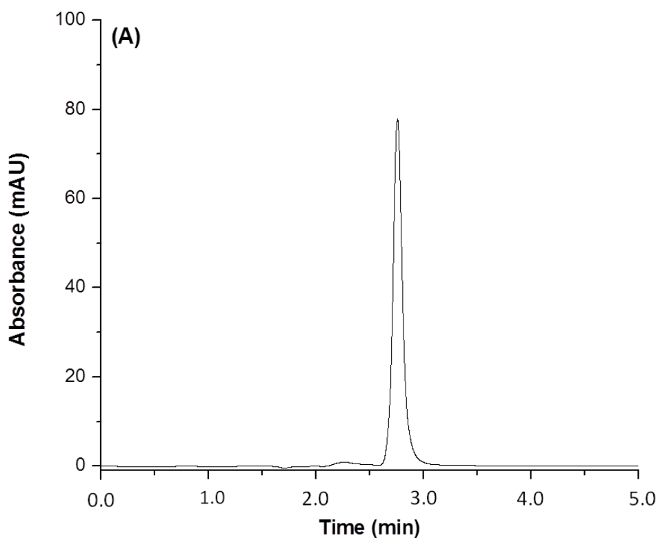
Figure S1. (A) HPLC Chromatogram of 16b ; (B) HPLC Chromatogram of 17b .
