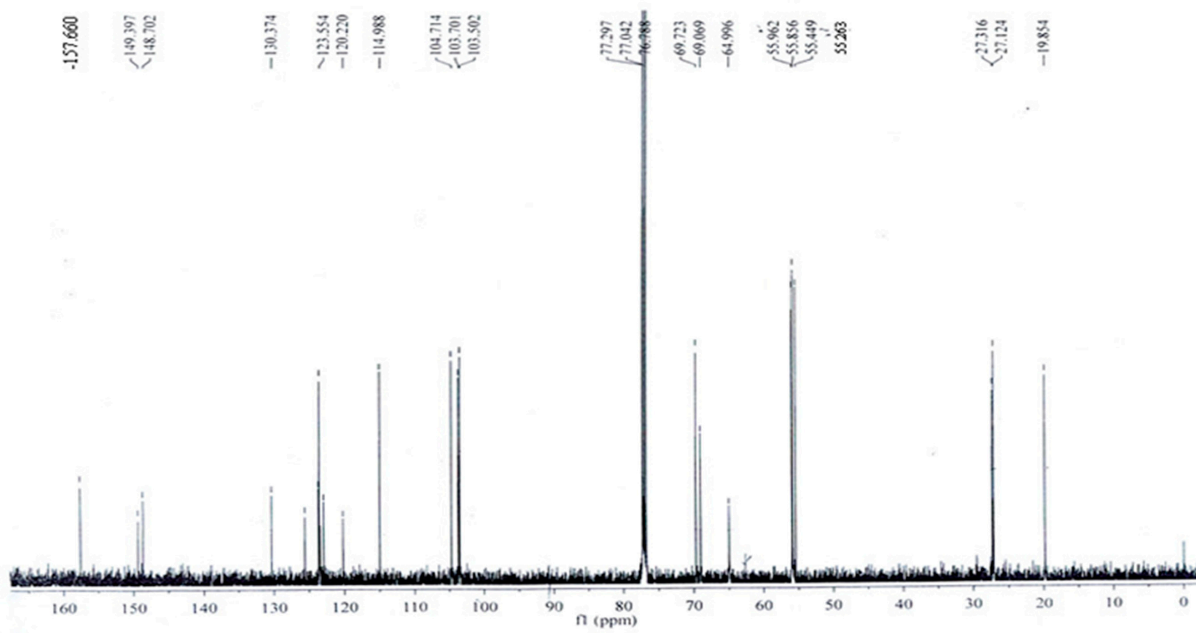
Figure S6. 1 H-NMR spectra of tylophorine.
