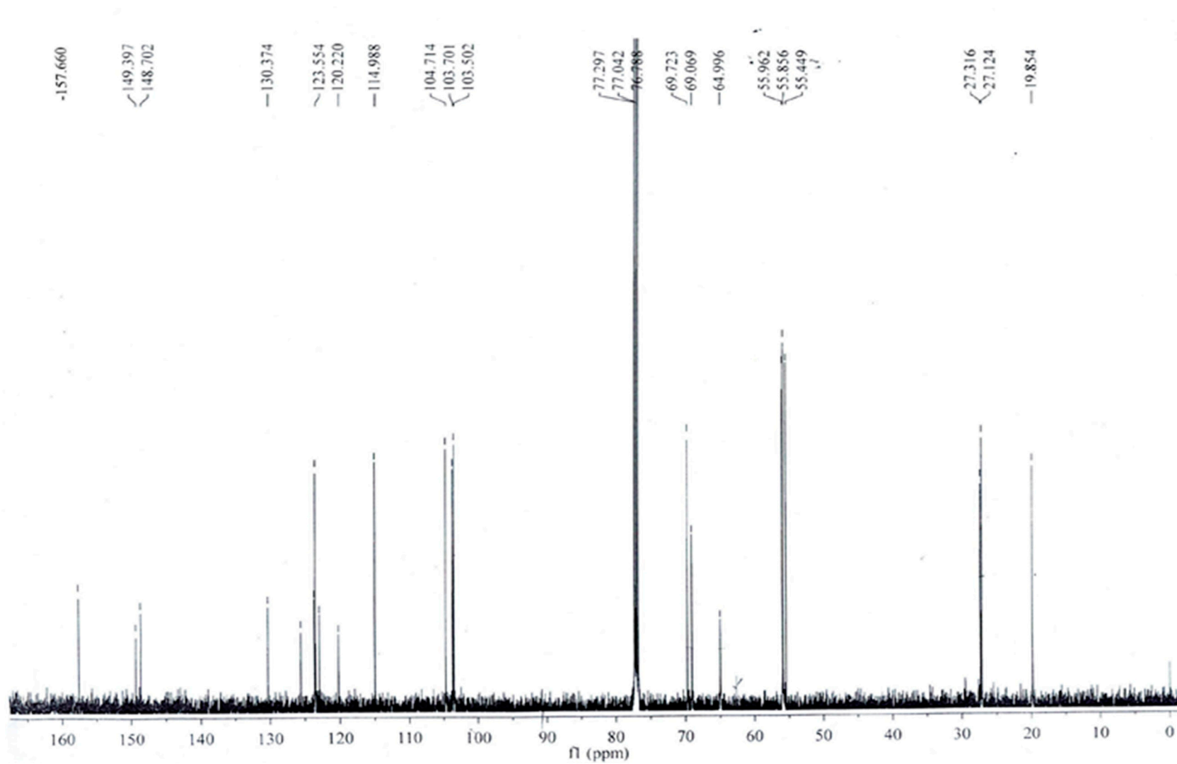
Figure S2. ^{13}\text{C} -NMR spectra of N -oxide antofine.
