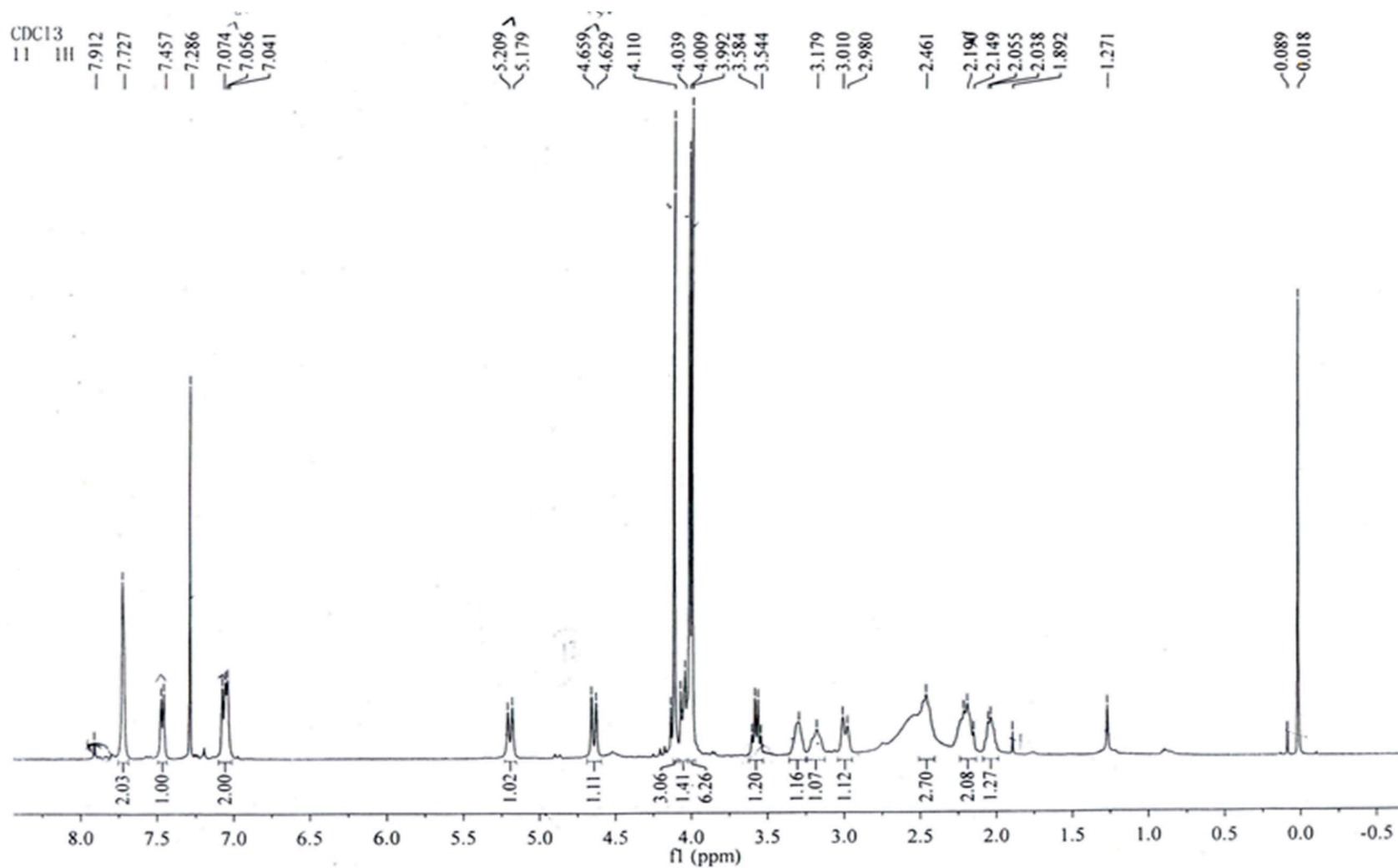
Figure S5. 13 C-NMR spectra of tylophorine.
