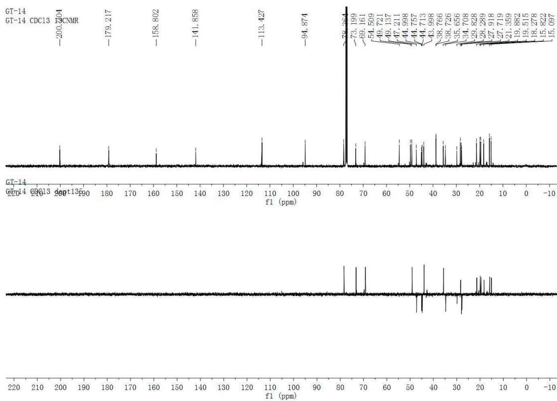
Figure S2. ^{13}\text{C} -NMR spectrum of compound 1 ( \text{CDCl}_3 , 125 MHz).
