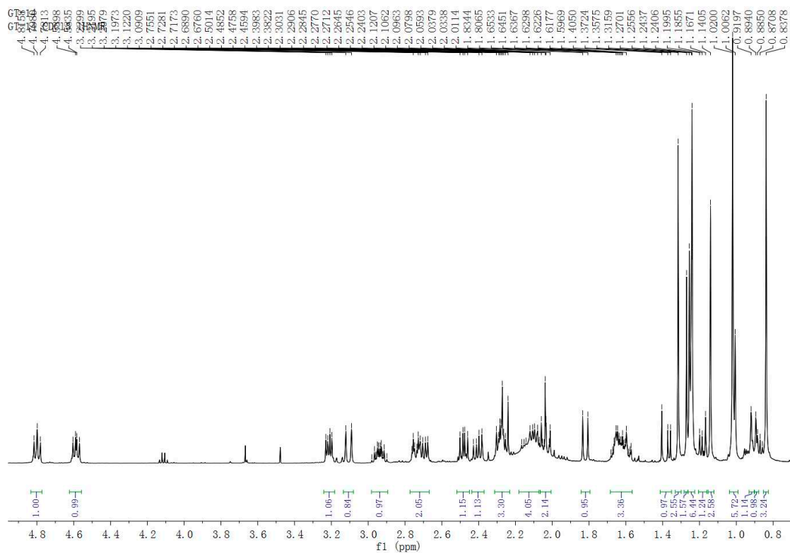
Figure S1. ^1\text{H} -NMR spectrum of compound 1 ( \text{CDCl}_3 , 500 MHz).
