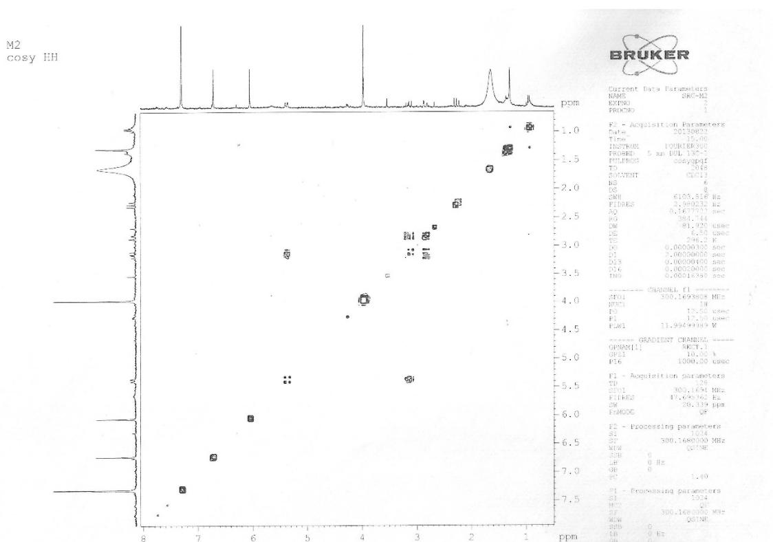
Figure S2. ^1\text{H} - ^1\text{H} COSY of compound 1.
