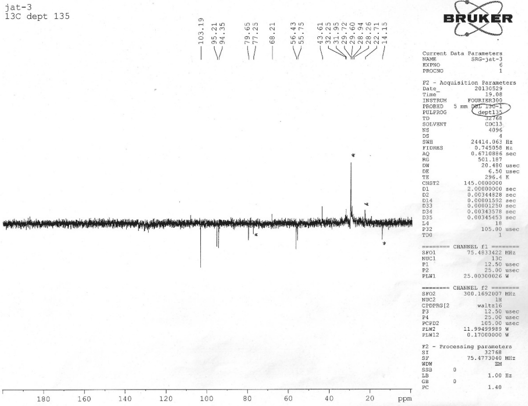
Figure S4. Dept 135 of compound 1.
