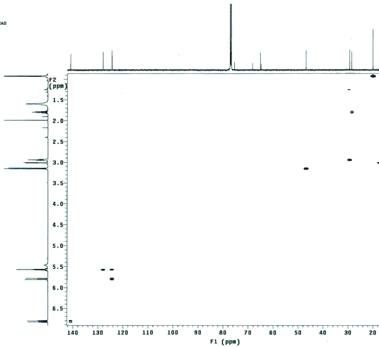
Figure S5. HMQC Spectrum of 1 in \text{CDCl}_3 .
