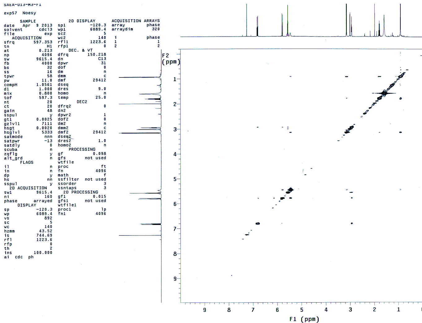
Figure S7. NOESY Spectrum of 1 in CDCl 3 .
