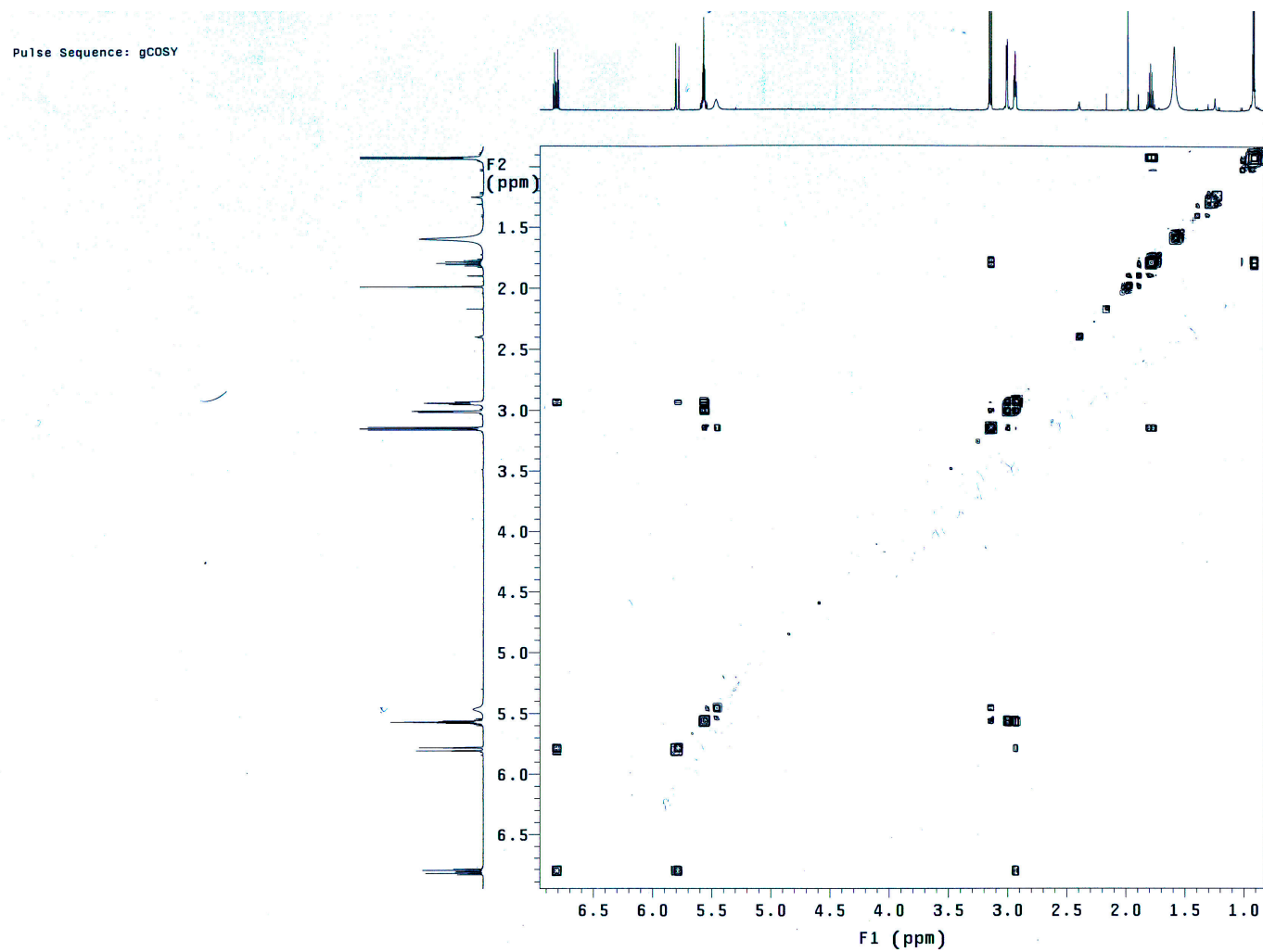
Figure S4. COSY Spectrum of 1 in \text{CDCl}_3 .
