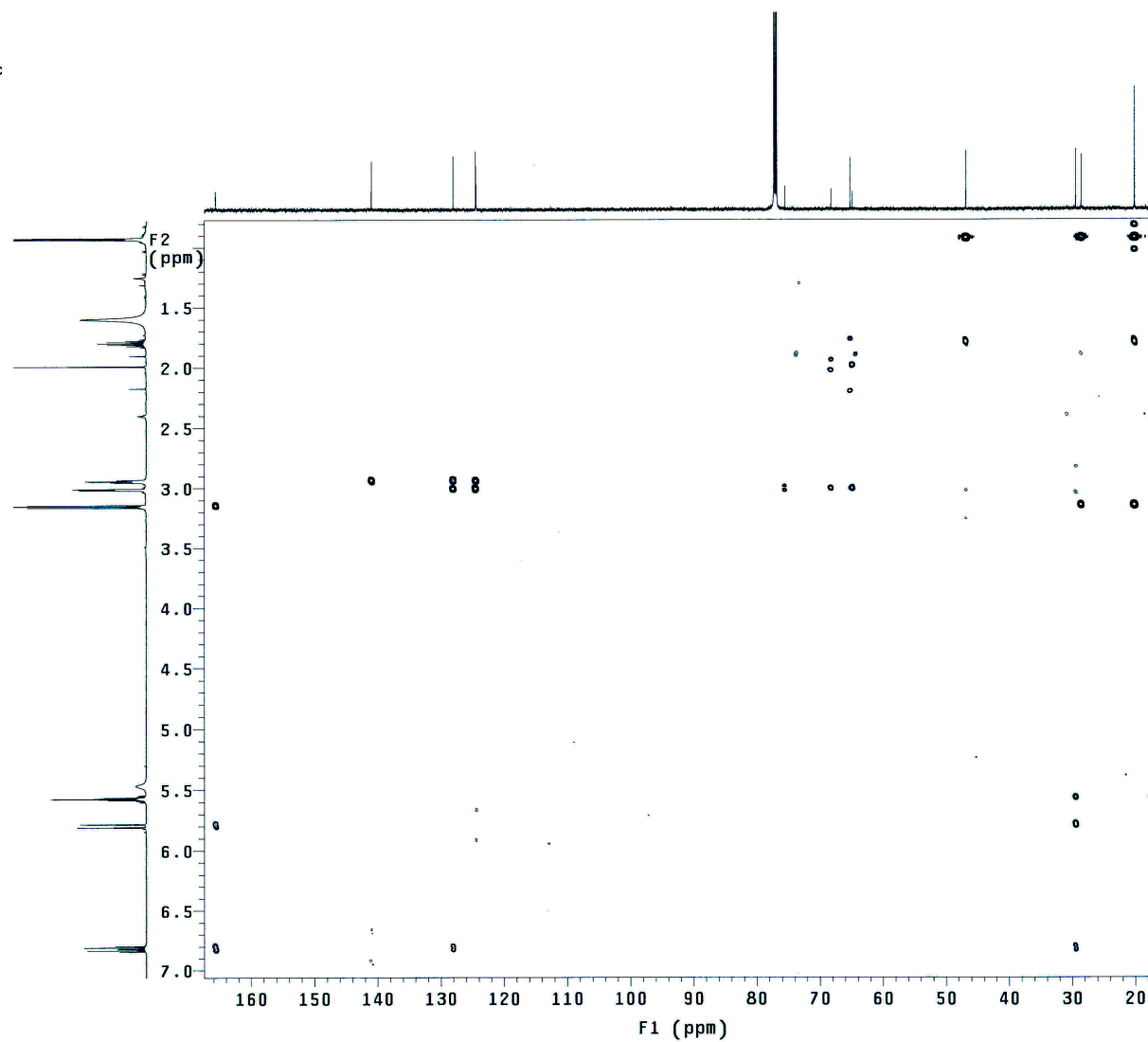
Figure S6. HMBC Spectrum of 1 in CDCl 3 .
