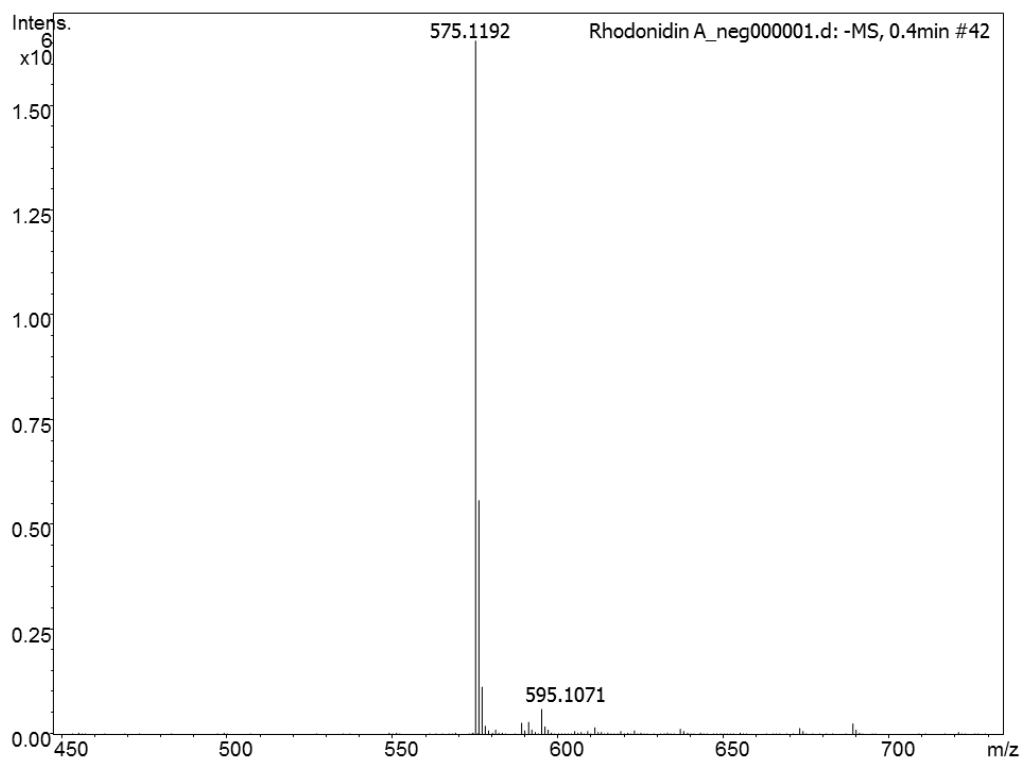
Figure S1. HR-ESIMS of 3
