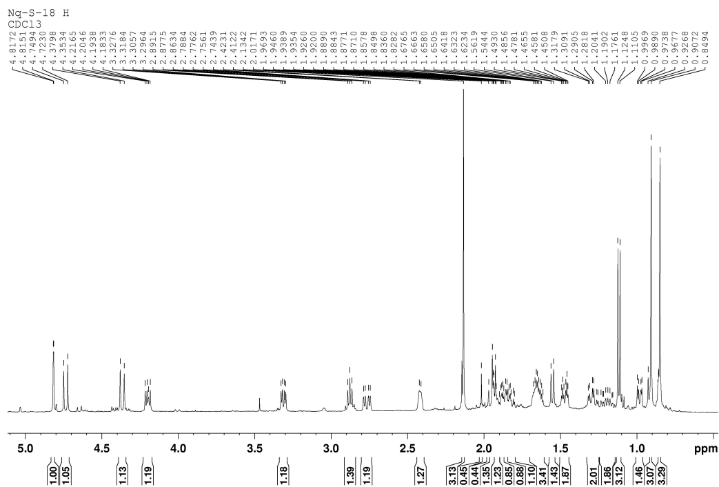
Figure S4. 1 H-NMR spectrum of compound 1.
