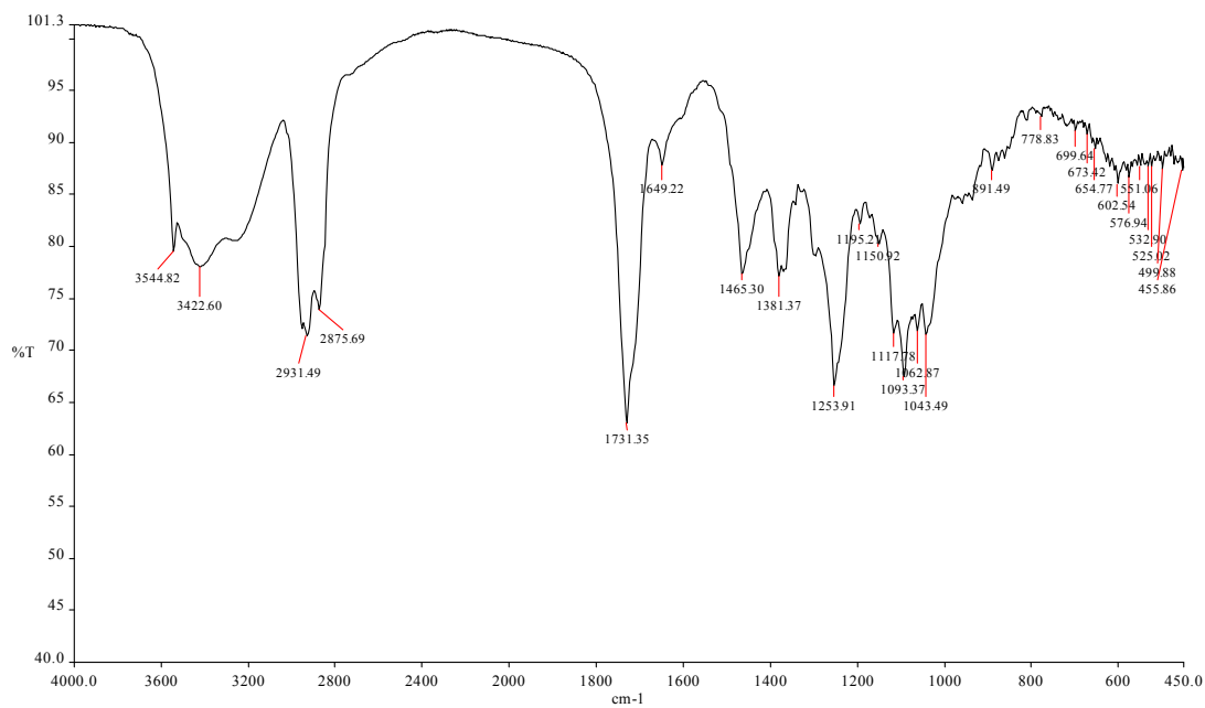
Figure S1. IR spectrum of compound 1.
