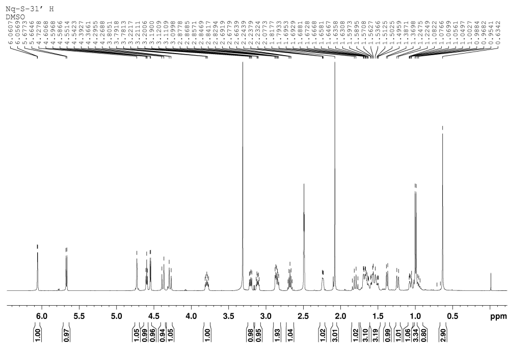
Figure S13. 1 H-NMR spectrum of compound 2.
