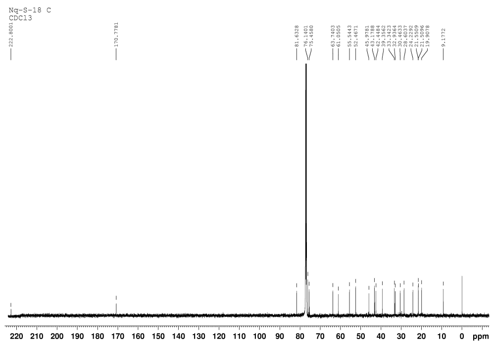
Figure S5. 13 C-NMR spectrum of compound 1.
