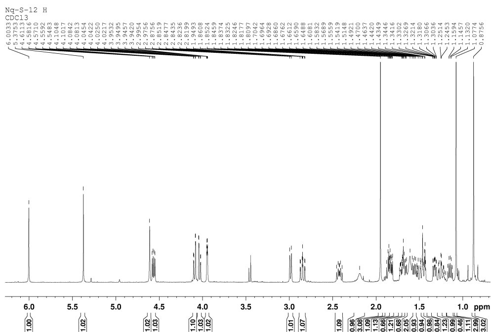
Figure S23. 1 H-NMR spectrum of compound 3.
