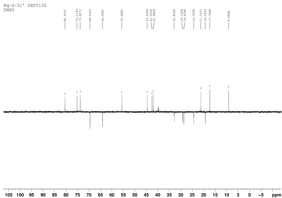
Figure S16. DEPT spectrum of compound 2.
