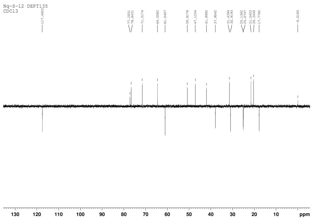
Figure S25. DEPT spectrum of compound 3.
