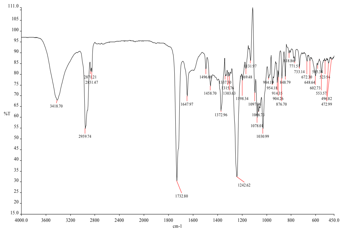
Figure S22. IR spectrum of compound 3.
