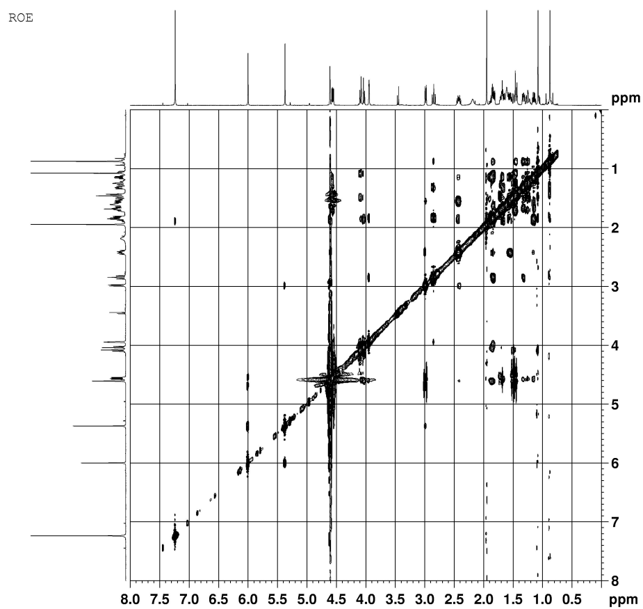
Figure S29. ROESY spectrum of compound 3.
