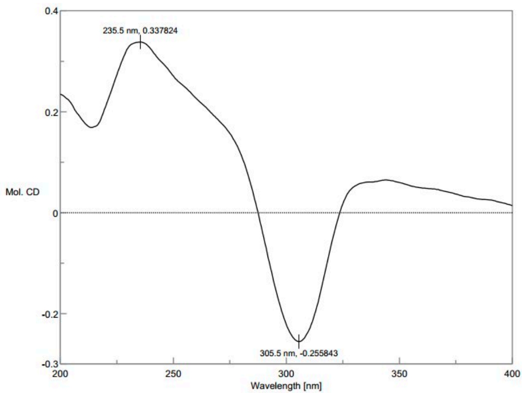
Figure S20. CD spectrum of compound 2.
