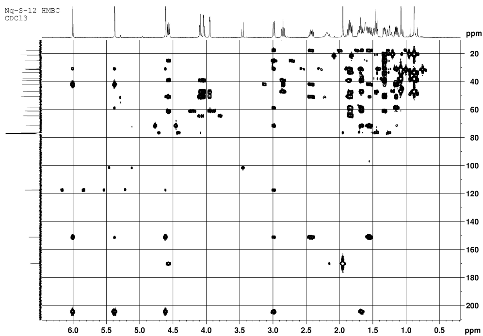
Figure S28. HMBC spectrum of compound 3.
