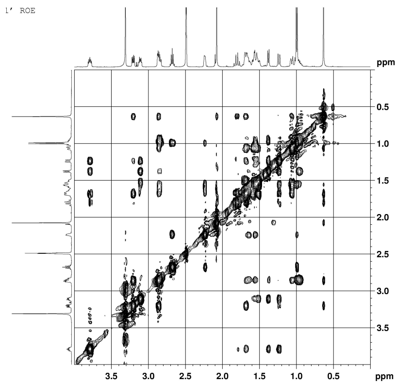
Figure S19. ROESY spectrum of compound 2.
