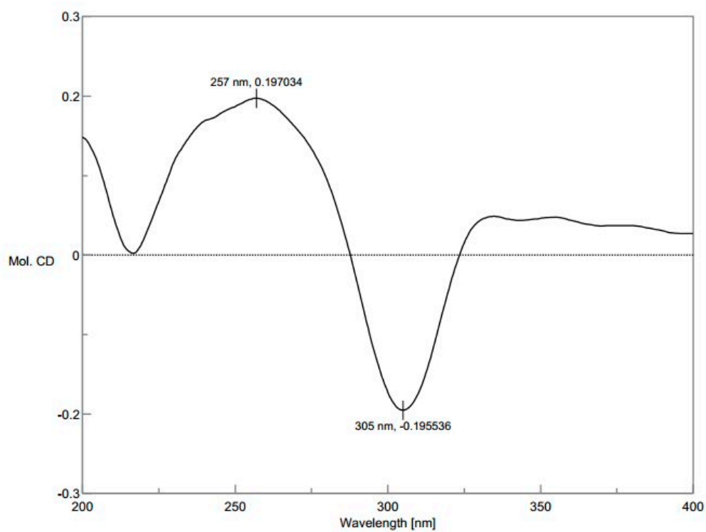
Figure S10. CD spectrum of compound 1.
