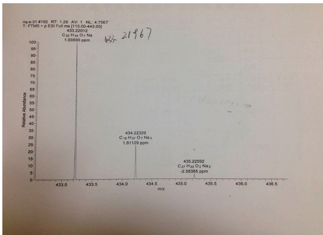
Figure S12. HR-ESI-MS spectrum of compound 2.
