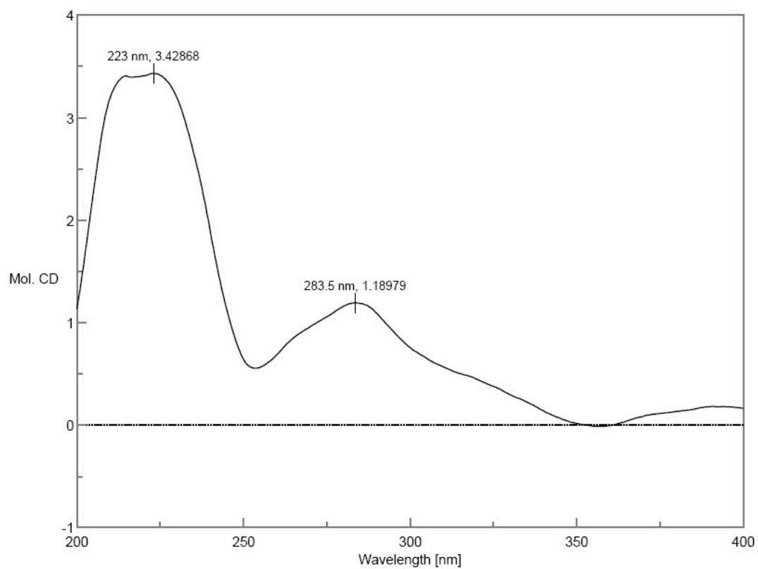
Figure S30. CD spectrum of compound 3.
