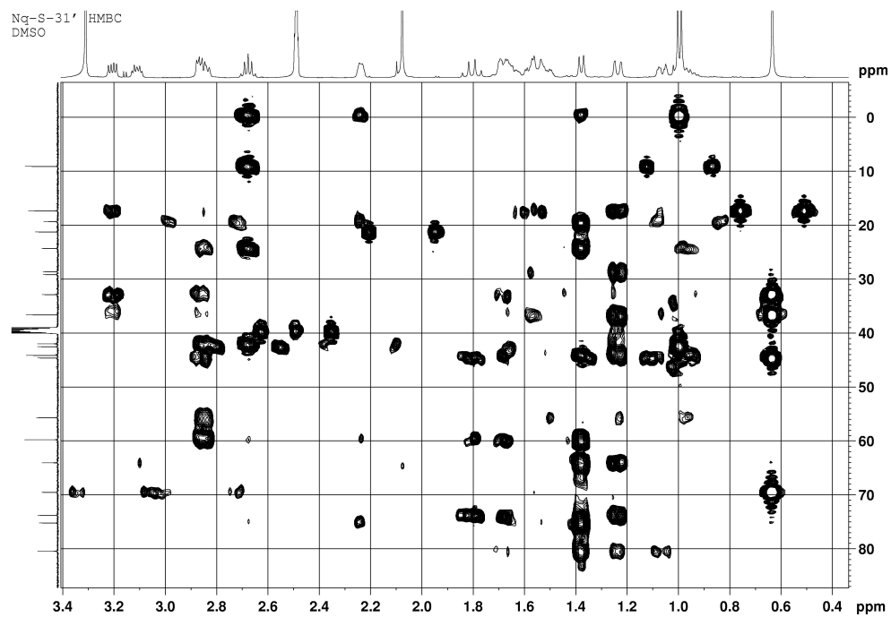
Figure S18. HMBC spectrum of compound 2.
