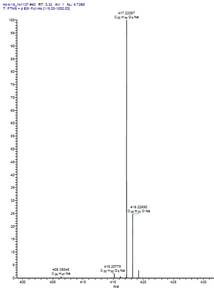
Figure S3. HR-ESI-MS spectrum of compound 1.
