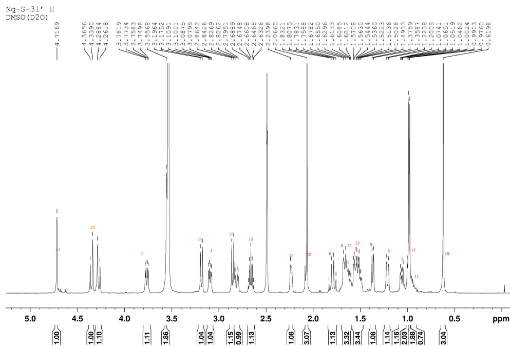
Figure S4. 1 H-NMR spectrum of compound 2.
