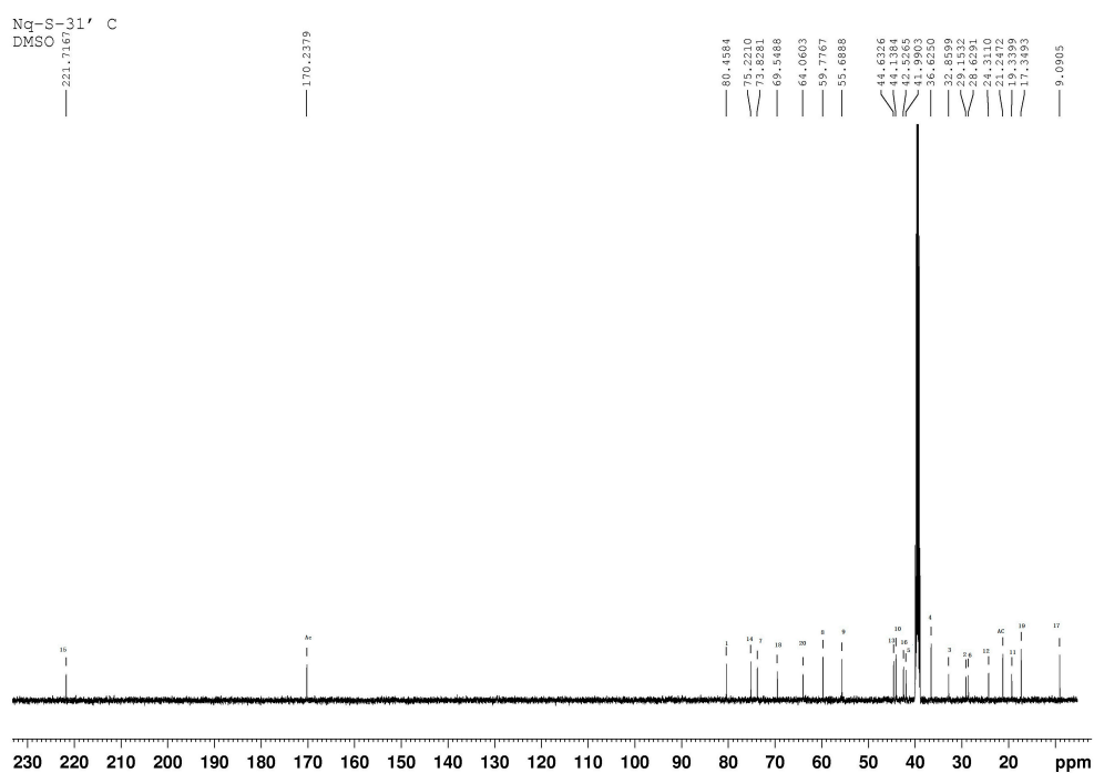
Figure S15. 13 C-NMR spectrum of compound 2.
