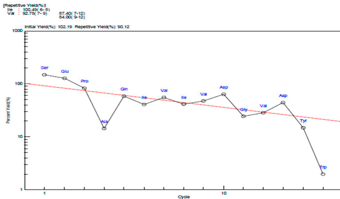
Figure S1. The amino acid sequence analysis of peptide SLP1.
