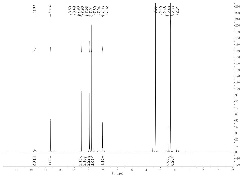
Figure S2. 1 H-NMR spectrum of HAMDC.
