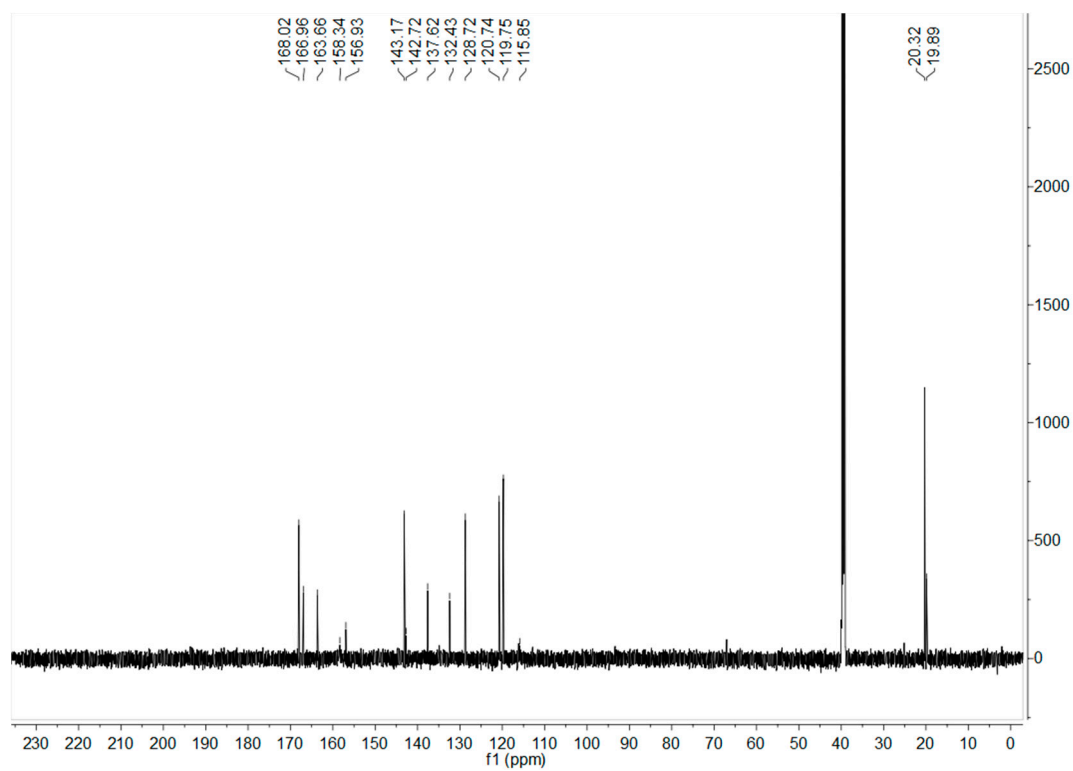
Figure S3. 13 C-NMR spectrum of HAMDC.
