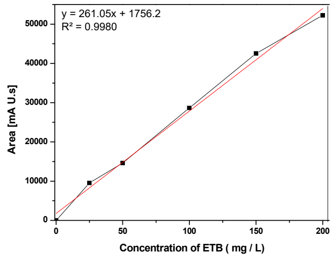
Figure S1. Calibration curve of ETB determined by using HPLC with different standard concentrations of 0 mg/L, 25 mg/L, 50 mg/L, 100mg/L, 150 mg/L, and 200 mg/L.
