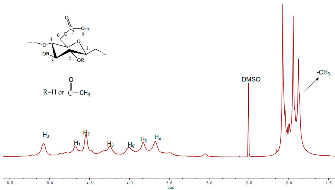
Figure S1. 1 H-NMR spectra of CA (DS=2.75).
