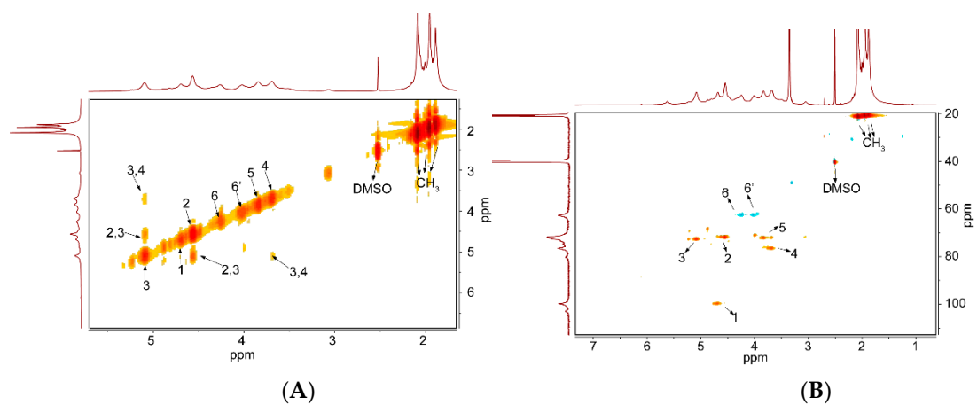
Figure S2. ^1\text{H} - ^1\text{H} COSY (A) and HSQC spectra (B) of the CA sample with DS of 2.75.
