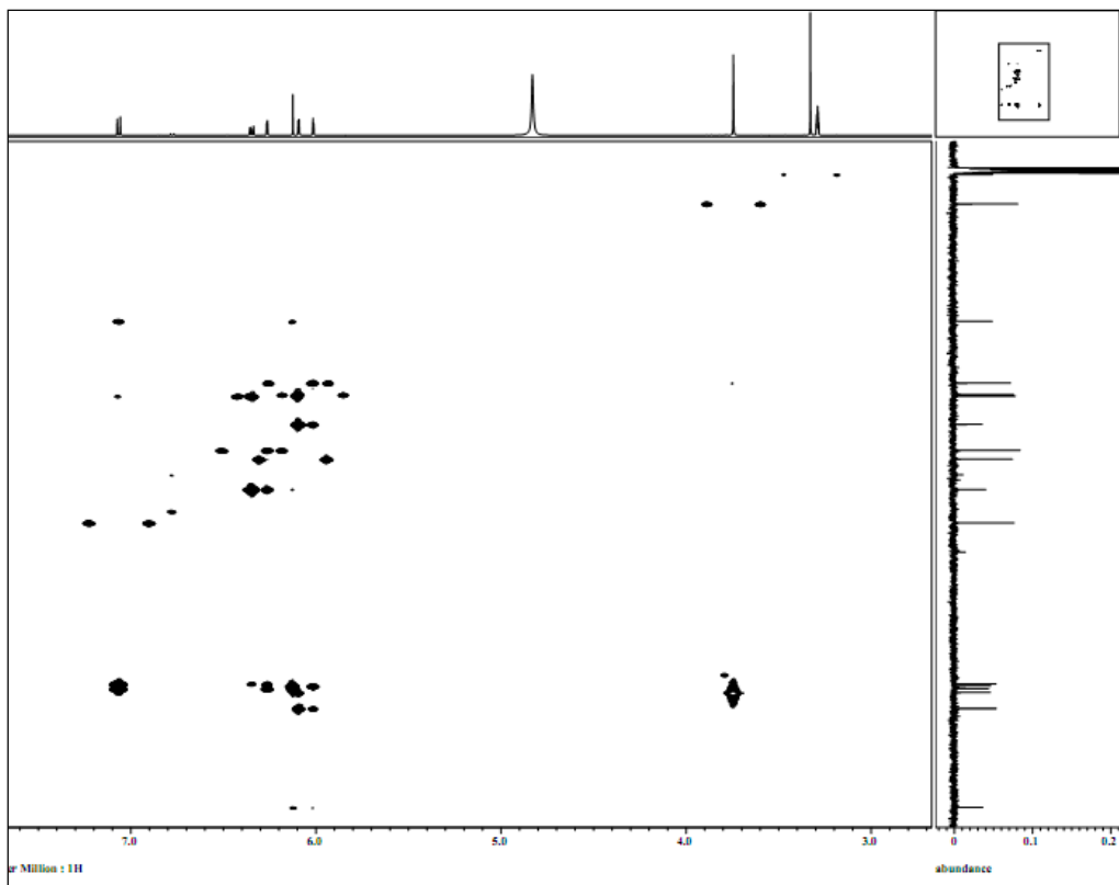
Figure S4. HMBC of compound 1.
