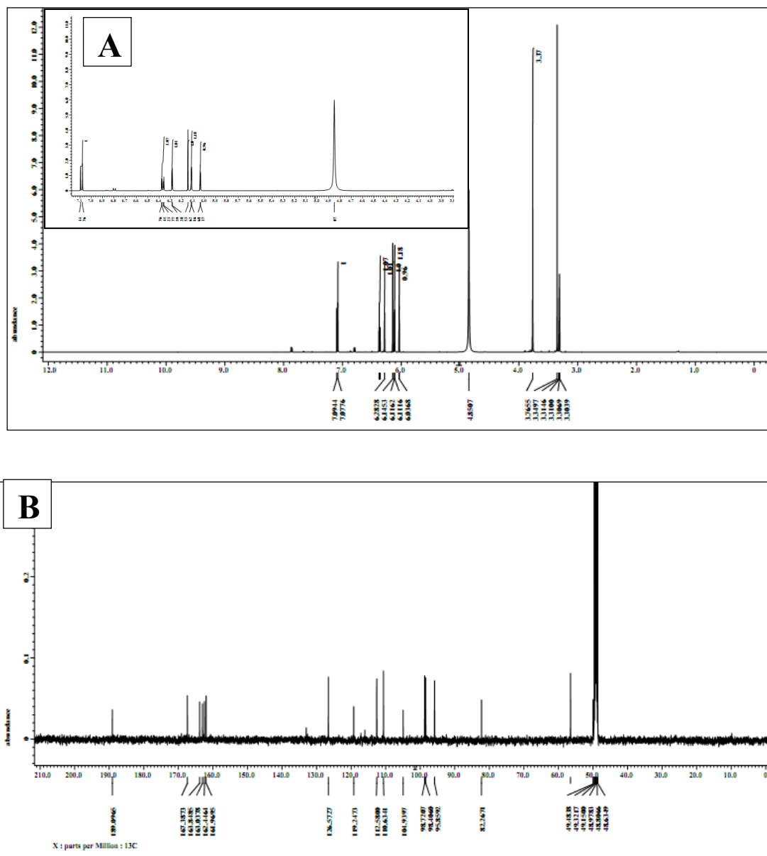
Figure S1. 1 H(A) and 13 C(B)-NMR of compound 1.
