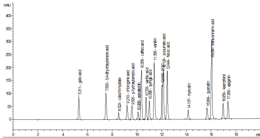
Figure 1S. HPLC chromatograms of 18 phenolic standard samples.
