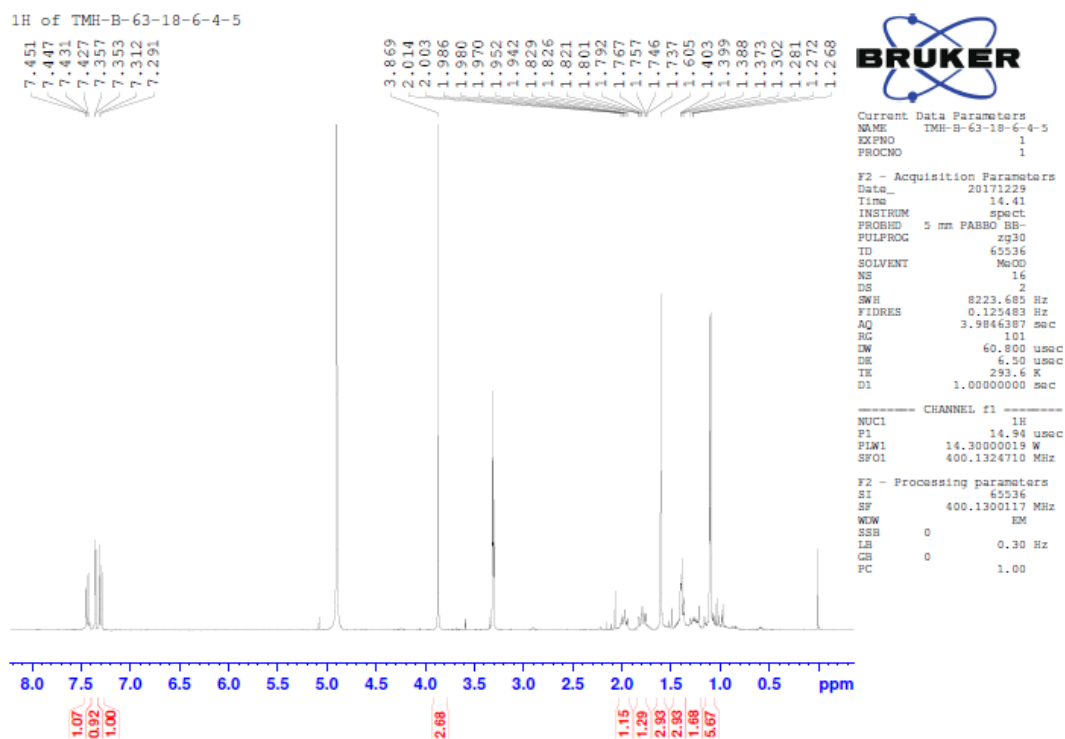
S5: the NMR spectra of compound 3 (Aspergoterpenin C)
