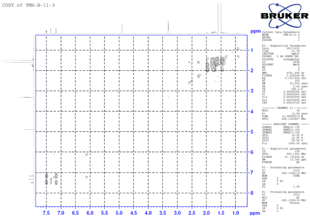
COSY of TMH-B-11-3
