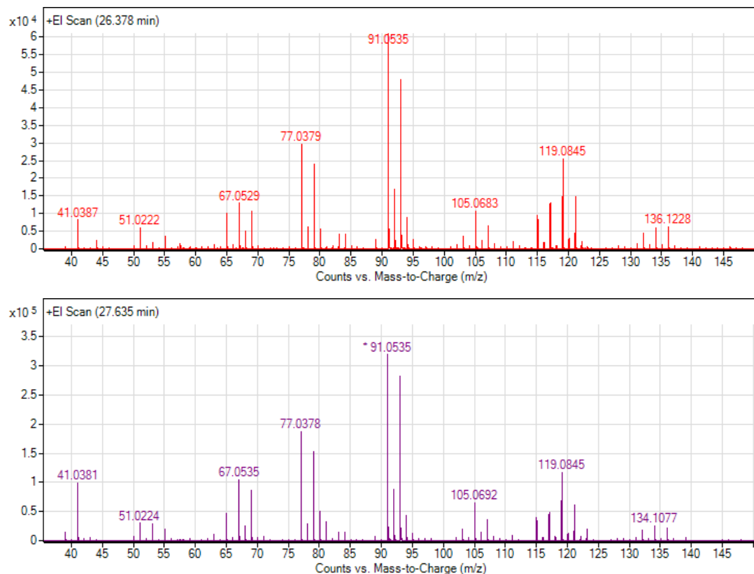
Figure S2 Mass spectra of unknown peak 1 and 2. The similar pattern indicated they were possibly isomers.
