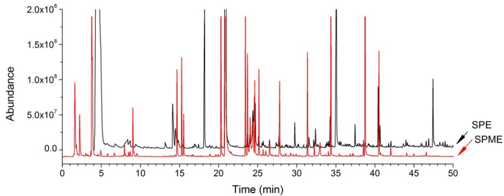
Figure S1 Example of separation and peak shape of O'Neal blueberry wine using SPE-GC-QTOF-MS and SPME-GC-QTOF-MS method.
