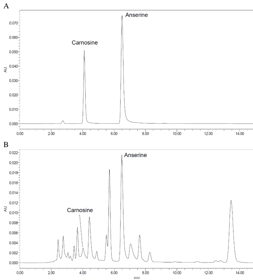
Figure S1. Typical HPLC chromatograms of (A) standard solution (250 mg/L) and (B) the extract of rainbow trout head.
