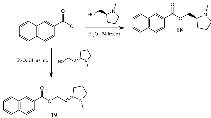
Figure S3.- Synthesis of 2-naphthoate derivatives (18-19).
