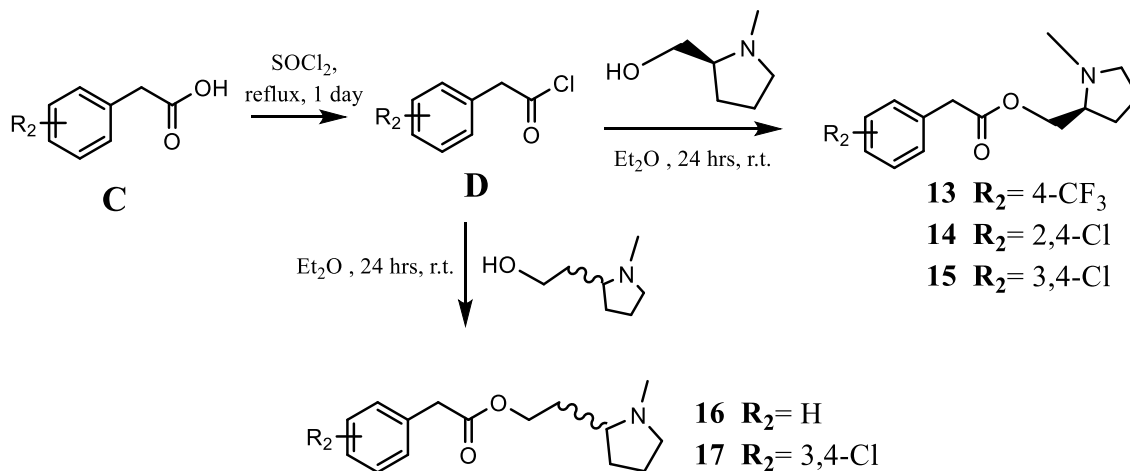
Figure S2.- Synthesis of 2-phenylacetate derivatives (13-17).
