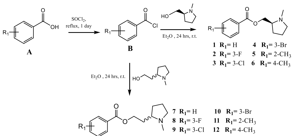
Figure S1.- Synthesis of benzoate derivatives (1-12).
