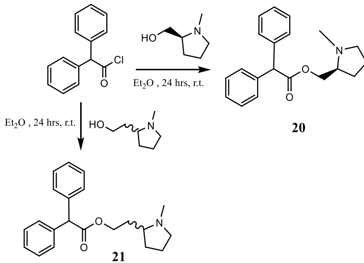
Figure S4.- Synthesis of 2,2-diphenylacetate derivatives (20-21).
