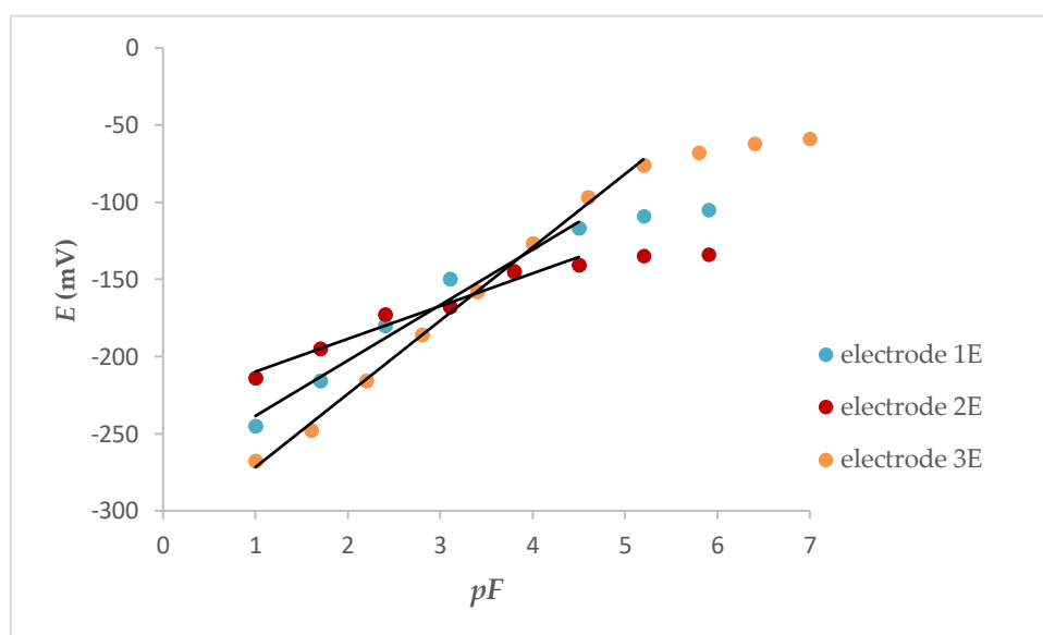
Figure S2. Potentiometric response of internal electrolyte contact \text{LaF}_3 electrodes before \text{Fe}_3\text{O}_4 NPs loading
