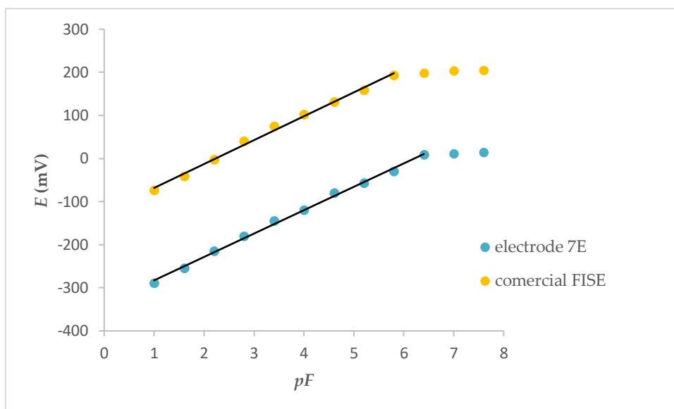
Figure S5. Calibration curves for fluoride determination with 7E and comercial FISE
