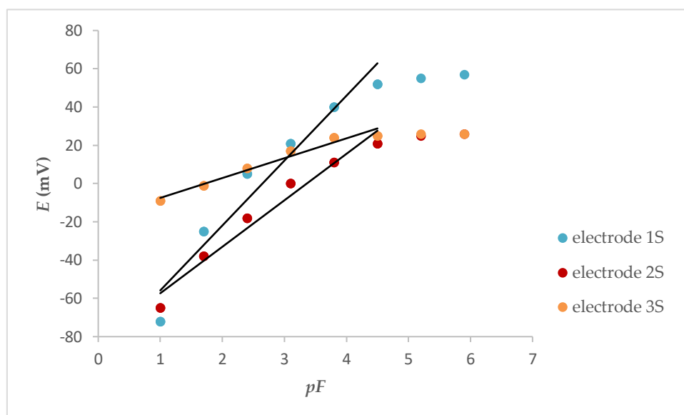
Figure S1. Potentiometric response of internal solid contact \text{LaF}_3 electrodes before \text{Fe}_3\text{O}_4 NPs loading
