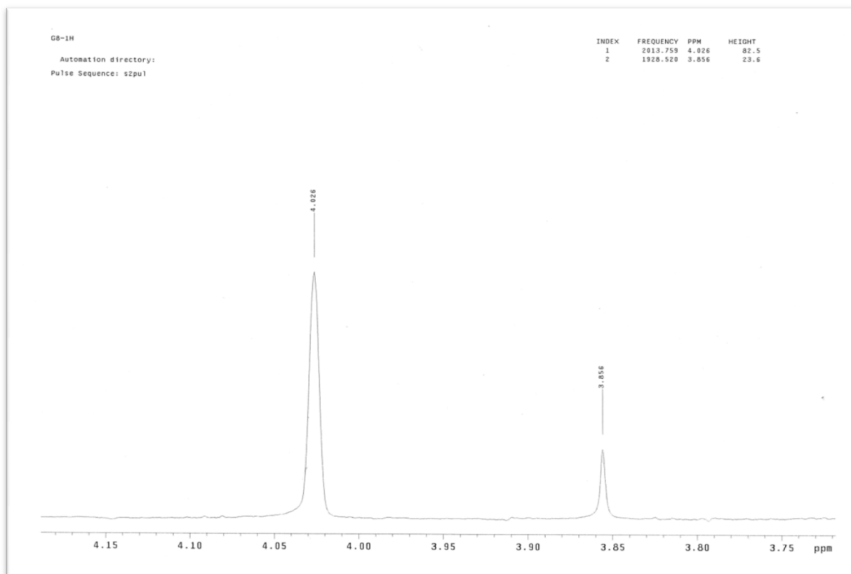
Figure S7. ^1\text{H-NMR} (500 MHz, \text{DMSO-}d_6 ) (Expanded 4).
