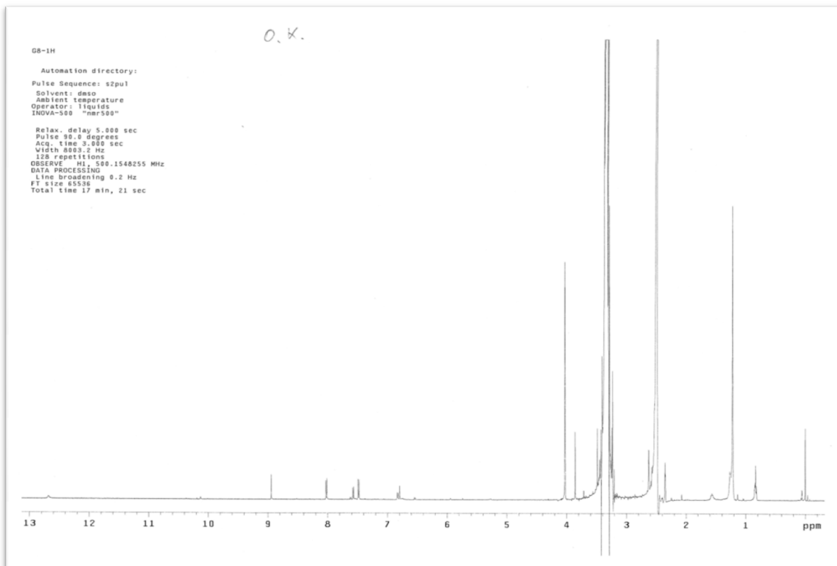
Figure S4. 1 H-NMR (500 MHz, DMSO-d 6 ) (Expanded 1).
