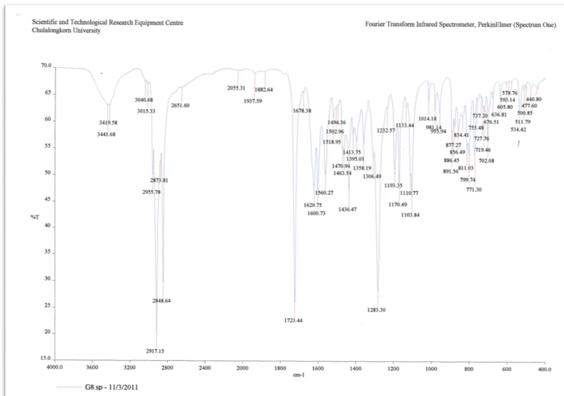
Figure S2. IR.
