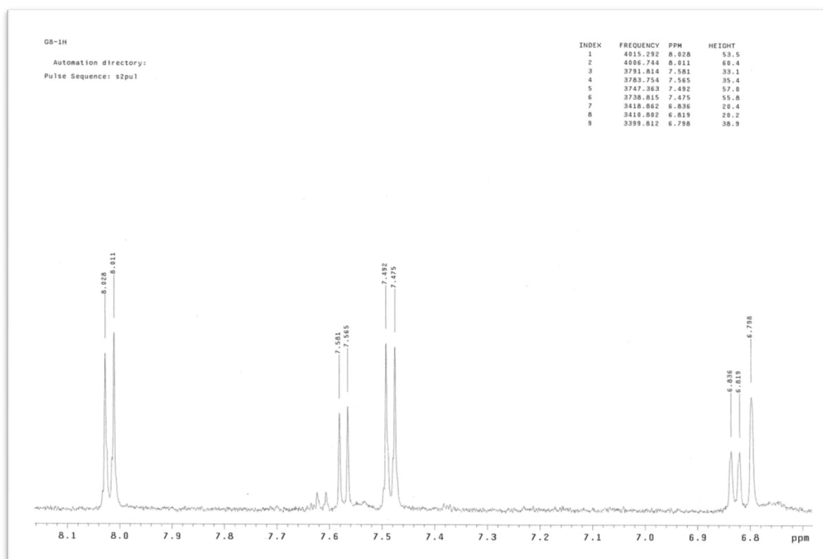
Figure S6. ^1\text{H-NMR} (500 MHz, \text{DMSO-}d_6 ) (Expanded 3).
