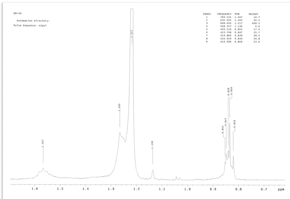
Figure S8. ^1\text{H-NMR} (500 MHz, \text{DMSO-}d_6 ) (Expanded 5).
