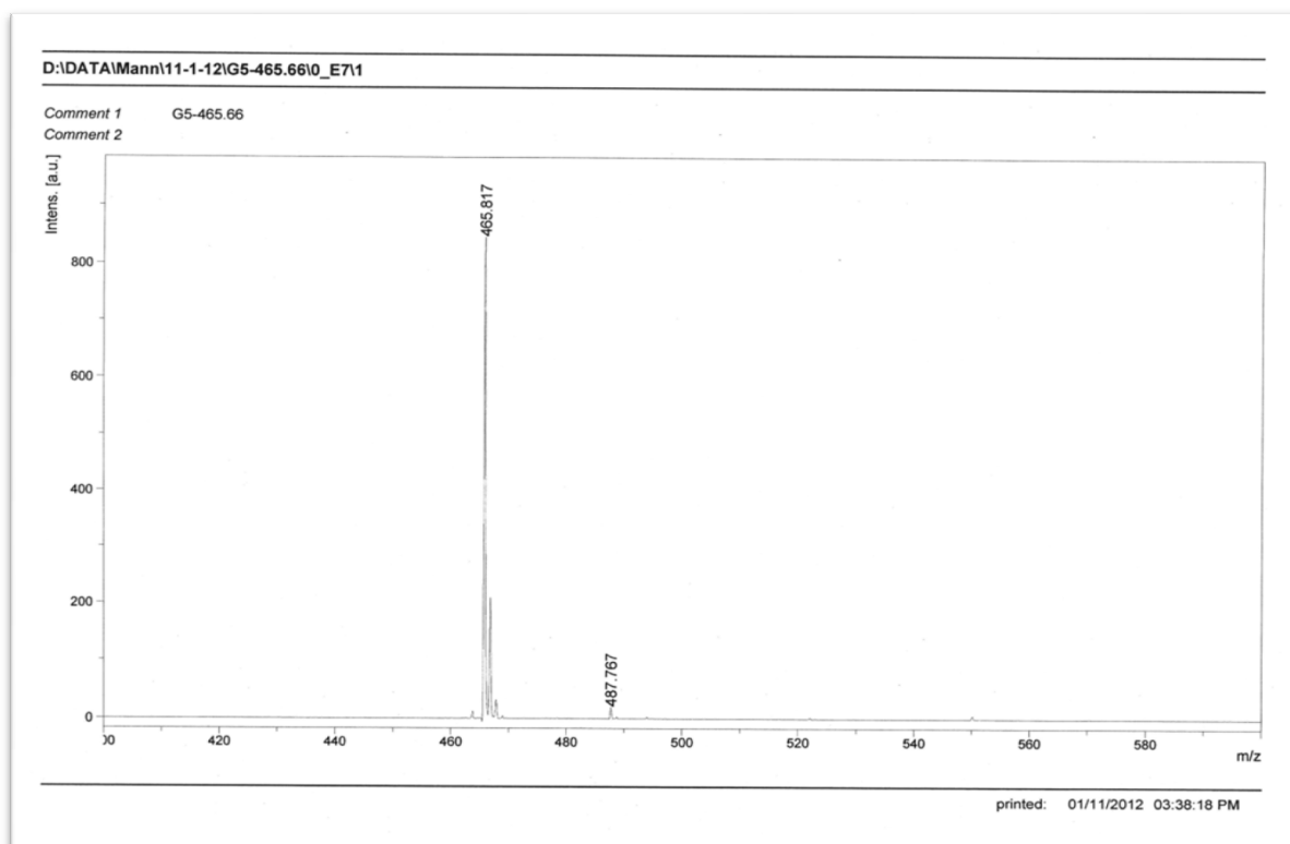
Figure S10. ESI-MS.
