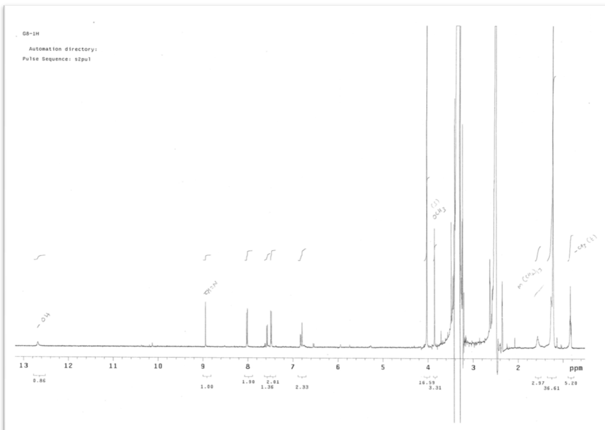
Figure S4. 1 H-NMR (500 MHz, DMSO-d 6 ) (Expanded 1).
