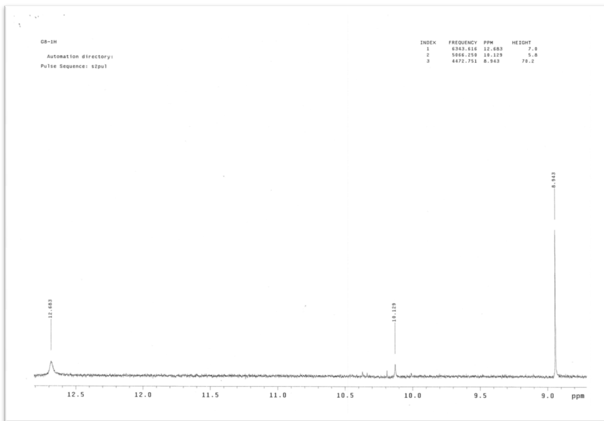
Figure S6. ^1\text{H-NMR} (500 MHz, \text{DMSO-}d_6 ) (Expanded 3).
