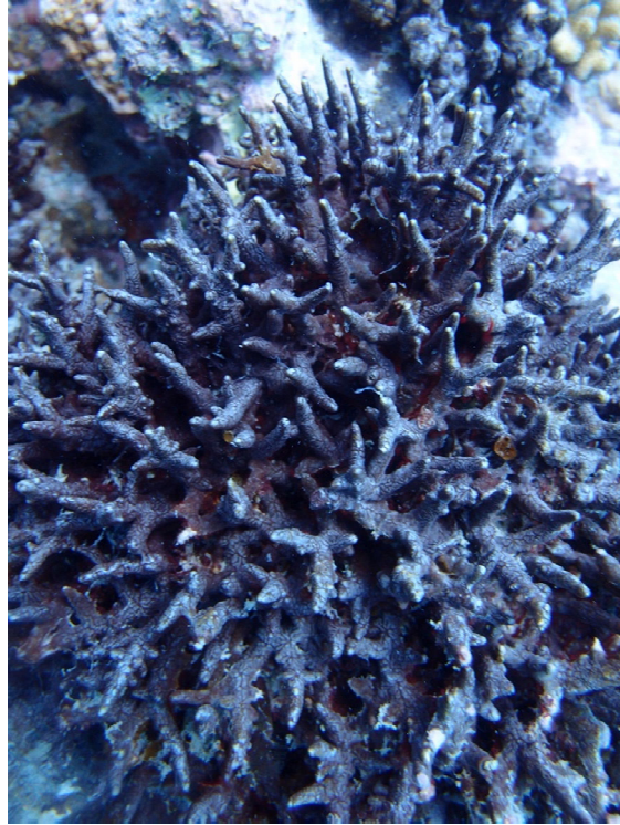
Figure S3. Putative Terpios hoshinota overgrowing a colony of Seriatopora hystrix at Heritage Reef (station 191).
