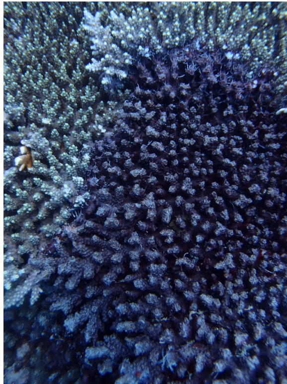
Figure S2. Putative Terpios hoshinota overgrowing a colony of Acropora latistella at Heritage Reef (station 191).
