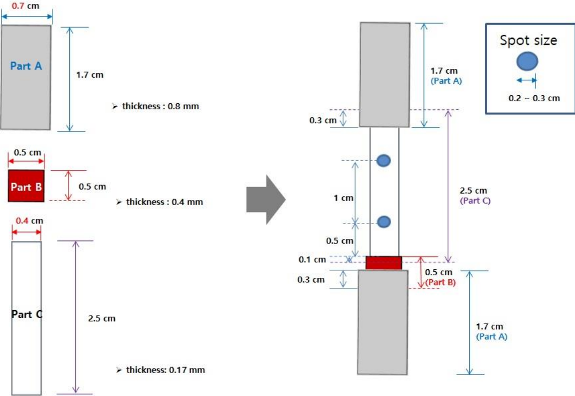
Figure 1. Schematic of immunochromatographic pepsin strip.
