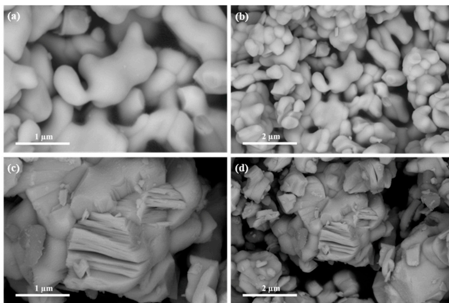
Figure S1. SEM images of \text{Bi}_4\text{Nb}_{0.9}\text{Zn}_{0.1}\text{O}_8\text{Cl} (a) (b); \text{Bi}_4\text{Nb}_{0.7}\text{Zn}_{0.3}\text{O}_8\text{Cl} (c) (d).
