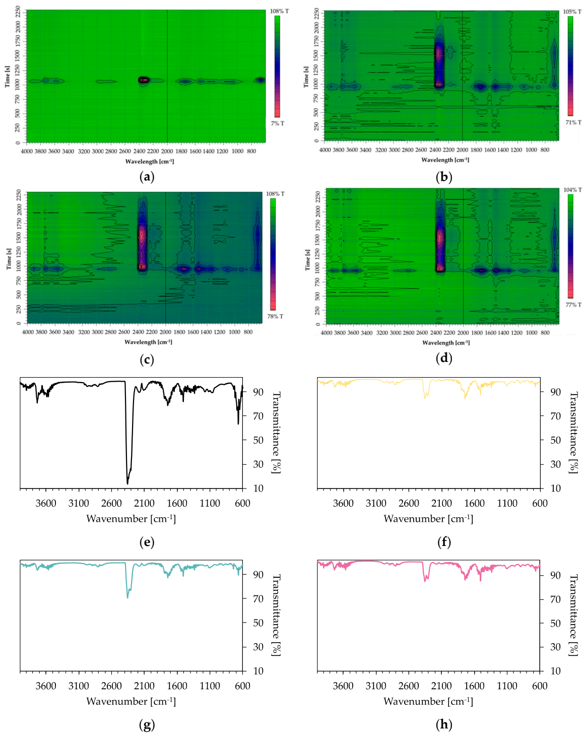
Figure S1. 2D plots and FTIR-spectra of the corresponding first peak maxima of uncoated and coated cotton fabrics, obtained by TGA-FTIR investigations in air. (a) 2D plot of uncoated cotton; (b) 2D plot of 5 BL; (c) 2D plot of 10 BL; (d) 2D plot of 15 BL; (e) spectrum at 1070 s (357 °C in TGA) of uncoated cotton; (f) 5 BL spectrum at 950 s (317 °C in TGA); (g) 10 BL spectrum at 970 s (323 °C in TGA); (h) 15 BL spectrum at 950 s (317 °C).
