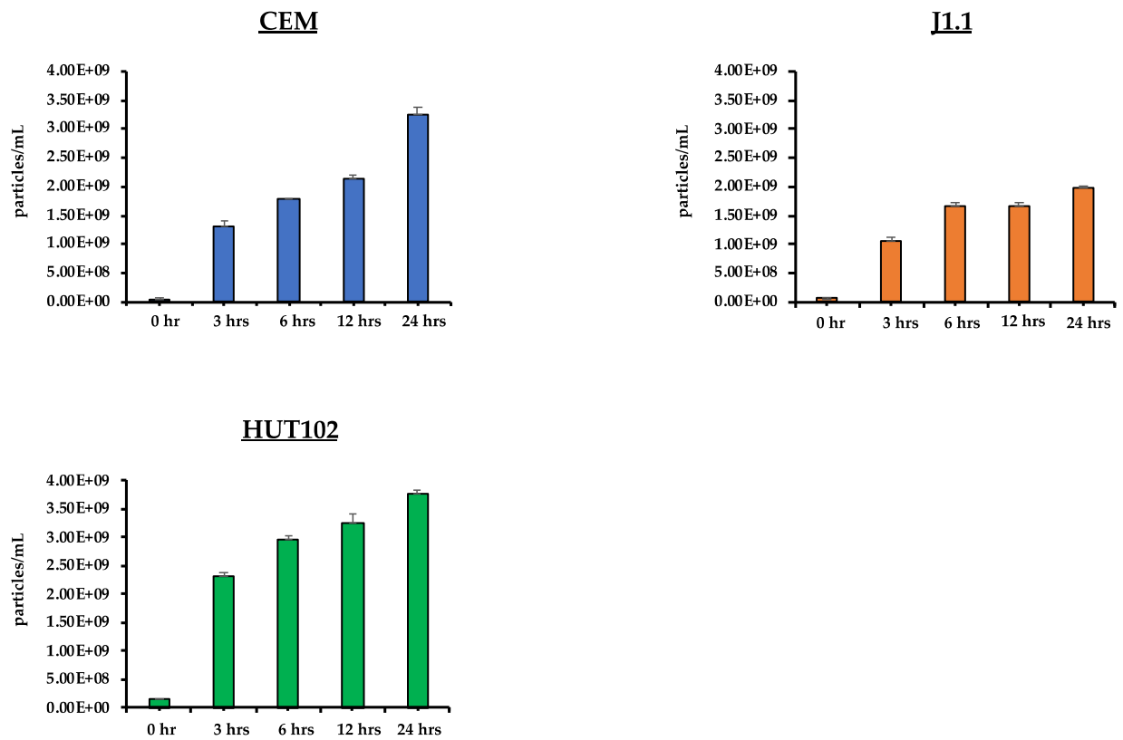
Figure S1. EV Concentration Increases Over Time. ZetaView analysis of supernatant material derived from uninfected (CEM), HIV-1-infected (J1.1), and HTLV-1-infected (HUT102) cells was performed to determine EV concentration from three technical replicates of 0-, 3-, 6-, 12-, and 24-h samples.
