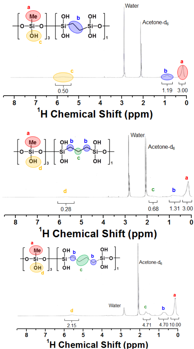
Figure S1. ^1\text{H} -NMR analysis of MTMS-BTES _n (75:25, mol%) copolymer.
