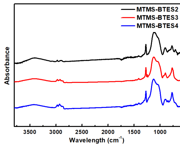
Figure S2. Fourier transform infrared spectroscopy (FT-ir) of MTMS-BTES n copolymer.
