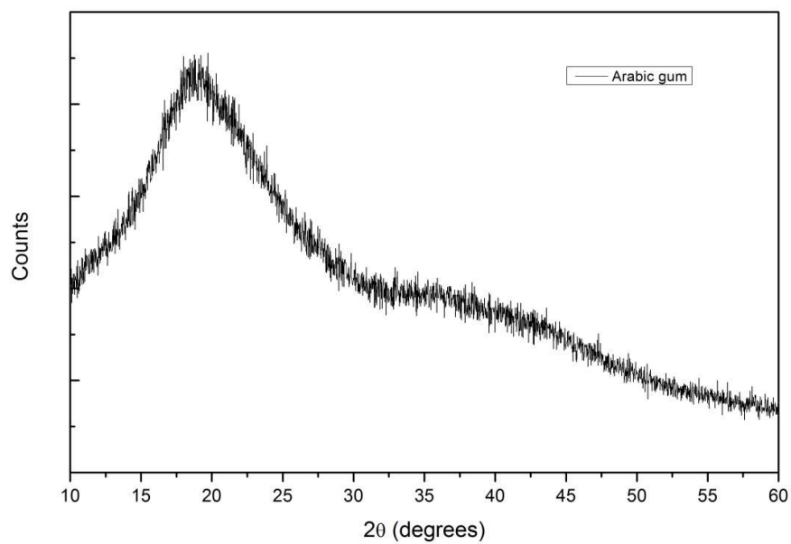
Figure S2. XRD diffractogram for Arabic gum.
