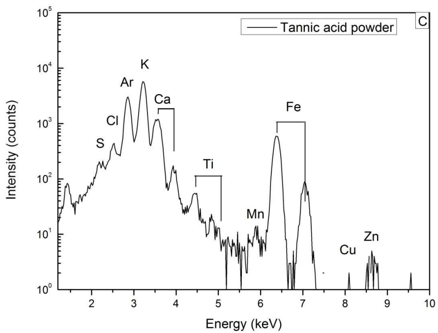
Figure S1. PIXE spectra of the ingredients. (A) Arabic gum; (B) iron sulfate; (C) tannic acid powder.
