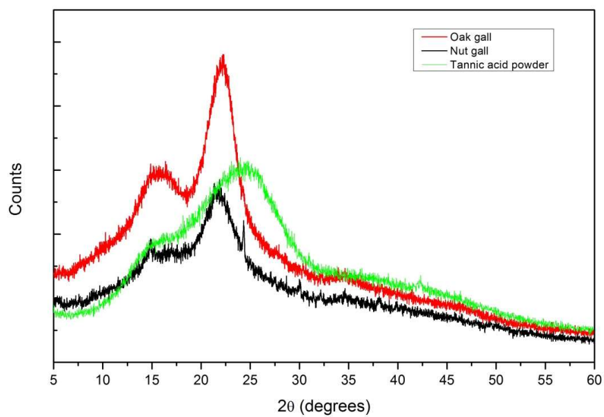
Figure S3. XRD diffractograms for tannin sources.
